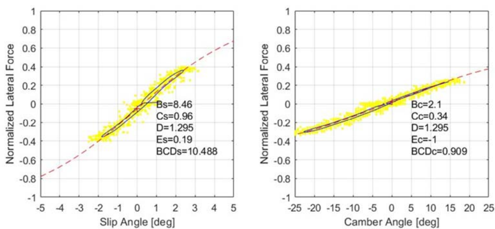
Figure 2: Example stiffness raw data, smoothed line, and fit curves for a particular tyre, rim, vertical load, and inflation pressure.
