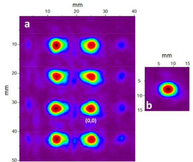
Fig. 1. Measured output beams of the grating in (a) and input beam in (b).
