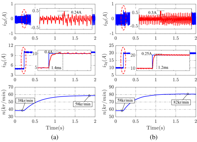
Fig. 7. Experimental results: MCF with proposed AD method. From top to down: i_{2d} , i_{2q} , and speed (kr/min).
