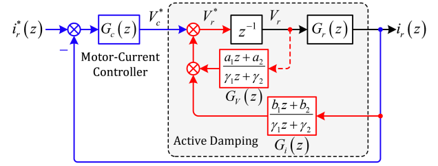
Fig. 2. Structure of the proposed general single-sensor AD method.
