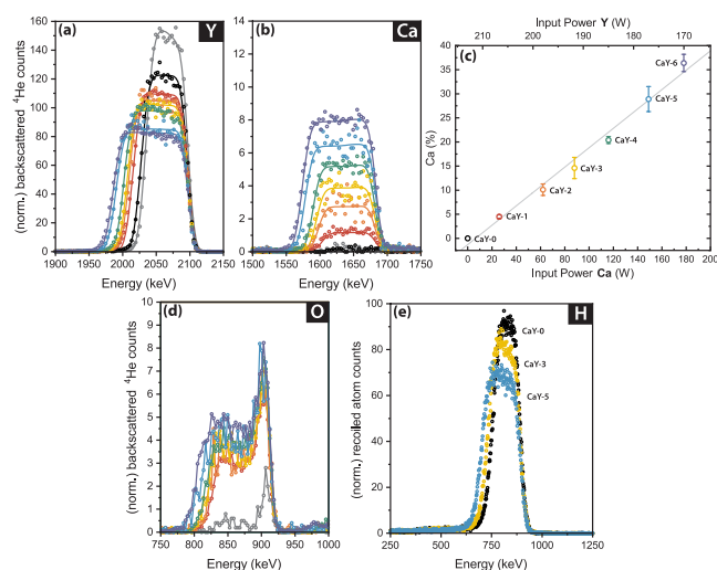
Figure 2. Overview of the compositions of Ca-doped oxyhydride thin films (\text{Ca}_x\text{Y}_{1-x})\text{H}_x\text{O}_y . For (a) and (b), the lines are from simulations of the composition using SIMNRA. RBS data for (a) yttrium, (b) calcium, and (d) oxygen are shown for \text{YH}_{1.9+\delta} and a series of oxyhydrides with gradually higher Ca content, where the black points are for CaY-0 (0% Ca) and the purple points are for CaY-6 with the most Ca. (c) The Ca content calculated from RBS along with the input power to the Ca and Y targets during cosputtering showing the linear relationship. (e) ERD results for hydrogen as more calcium is added to yttrium oxyhydride. All RBS and ERD data are normalized to account for differences in accumulated charge.
