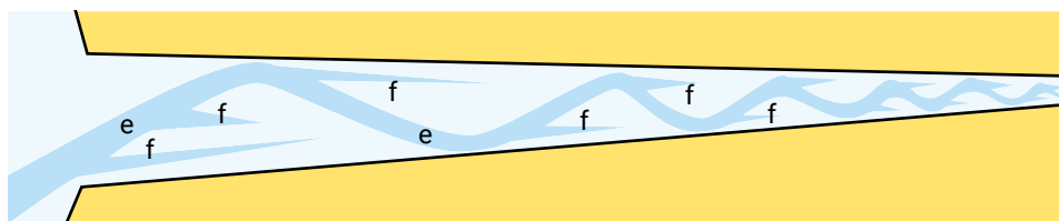
Figure 9.9: Sketch of an ideal system of ebb (e) and flood (f) channels (Scheldt estuary). It has a meandering main (ebb) channel and flood channels starting in every bend. The latter have a double function; viz. 1. filling the tidal sand flat in the inner bend of the main channel; 2. serving the cut-off current of the bend. After Van Veen et al. (2005).
