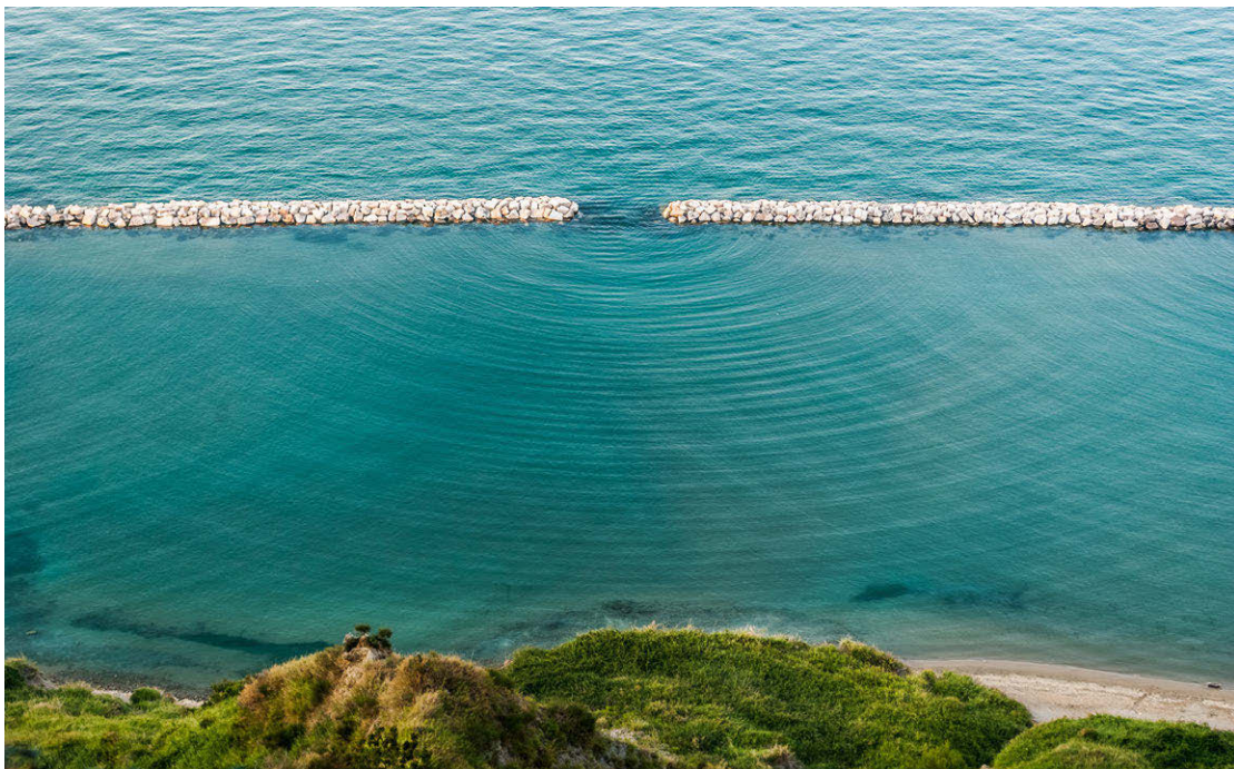
Figure 5.8: Typical diffraction pattern through a gap between two detached breakwaters in Pesaro, Italy. Photo by Roberto Lo Savio ('Credits' on page 575).
