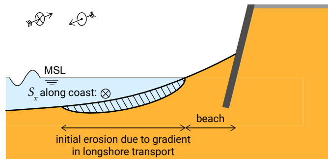
Figure 10.25: Seawalls and revetments cannot prevent structural erosion due to longshore transport gradients, since the longshore transports and transport gradients occur below the waterline in the surf zone.
