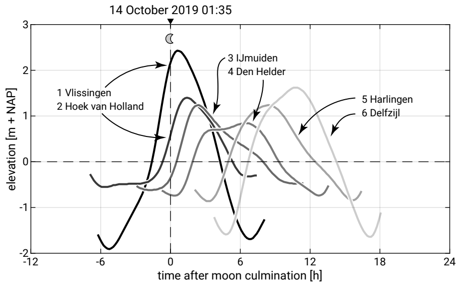
Figure 5.55: Tidal curves at six stations along the Dutch coast (data source: https://waterinfo.rws.nl/ ). The station numbers rise from south to north. The time in hours on the horizontal axis is relative to the moon culmination on October 14 th 2019 01:35 (calculated using https://www.mooncalc.org ). Note that MSL is approximately equal to NAP; current MSL is less than 0.1 m above NAP.
