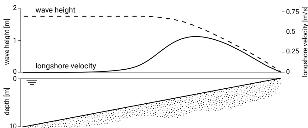
Figure 5.41: Wave-driven velocity computed with the computer model Unibest-CL+ ( https://www.deltares.nl/en/software/unibest-cl ) using as model input: H_{s,0} = 2 m; \gamma = 0.7 ; \varphi_0 = 30^\circ ; T_p = 8 s).
