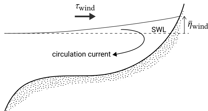
Figure 5.50: Wind set-up balancing wind shear stress in the case of onshore wind on a shelf. In the deep ocean, the water set into motion in the upper layers can easily spread out. Vertical exchange of water makes this possible. On the shelf there is no escape due to limited water depth and the surface water is driven ashore.
