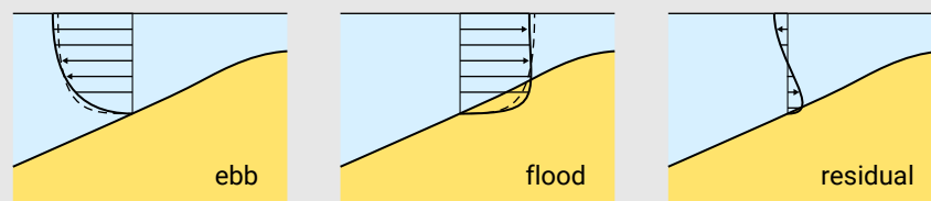
Figure 6.15: Residual tide-averaged velocity profile resulting in a net upslope transport.
