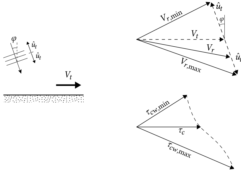
Figure 6.14: Left: plan view of velocity components u_t and V_t at a certain elevation z_t above the bed. Top right: the resultant velocity is V_r and varies in magnitude and direction during the wave cycle (between V_{r,min} and V_{r,max} ). Bottom right: bed shear stress components during the wave cycle. Since \tau_{cw} \propto |V_r| V_r , the larger velocities contribute relatively more to the bed shear stress.
