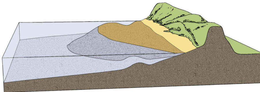
(c) mega-nourishment
