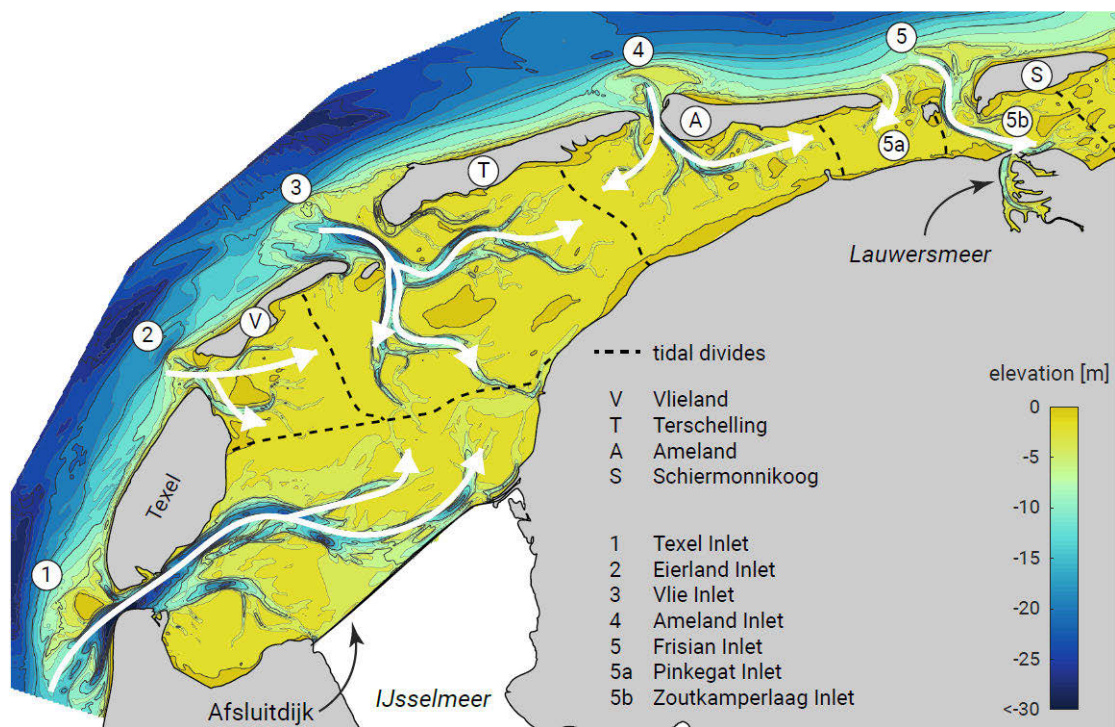
Figure 9.5: Wadden Sea tidal dynamics model, displaying the types of tidal passes and the wan-tide zones. The movement of the tide on the North Sea is from left to right.
