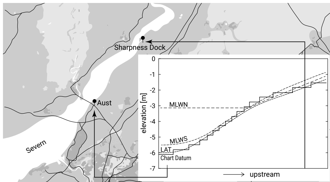
Figure C.1: River Severn (England). When CD is related to LAT, or another tidal level, it increases in upstream direction.
