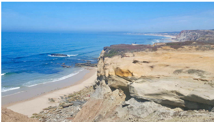
Figure 2.16: Cliffs with stacks at the coast of Peniche, Portugal. Photo by Ascha Simons ('Credits' on page 575).
