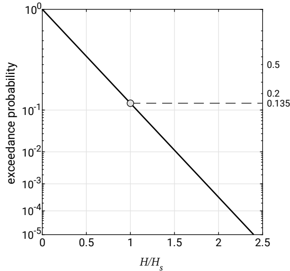
Figure 3.8: The exceedance probability P(H' > H) (Eq. 3.20) as a function of H/H_s shows as a straight line when plotted using a vertical scale with a spacing proportional to \sqrt{-\ln P} .
