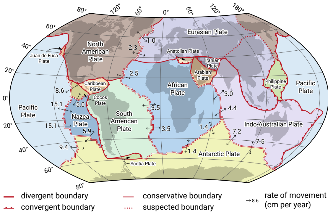
Figure 2.2: Movements of the tectonic plates: colliding or converging plates, diverging plates and plates grinding past each other (conservative or transform boundaries).
