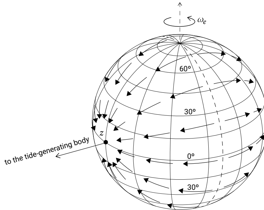
Figure 3.19: The horizontal component of the tidal force on the earth when the tide-generating body (the sun or the moon) is above the equator at z .
