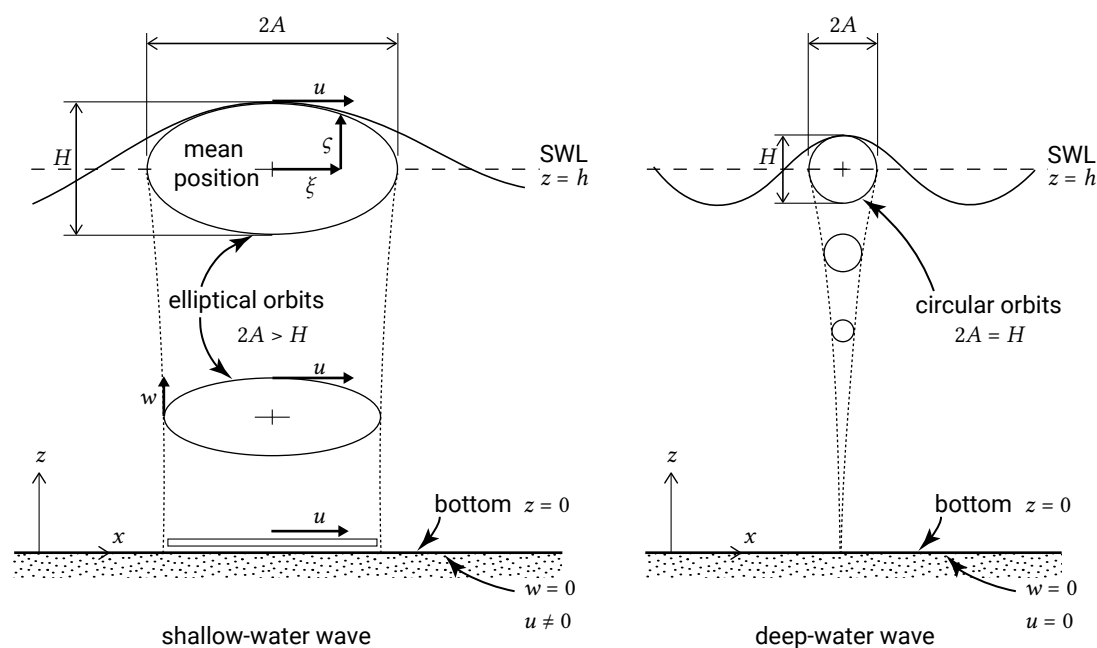
Figure A.2: Orbital motion under a shallow-water wave and a deep-water wave. Note that, as opposed to the definitions in Chapters 3 and 5, z = 0 at the bottom (instead of z = -h ) and z = h at the mean water level (instead of z = 0 ).
