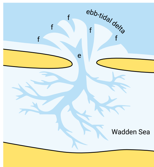
Figure 9.7: Sketch of ebb and flood channels in a typical Wadden Sea basin with an inlet between dune-islands, several flood channels coming in (indicated with f) and an ebb channel (e) and delta with a tendency to turn to the left, due to the ebb tide leaving to the left, consistent with the propagation direction of the tidal wave along the Dutch coast (see Fig. 3.31). After Van Veen et al. (2005).
