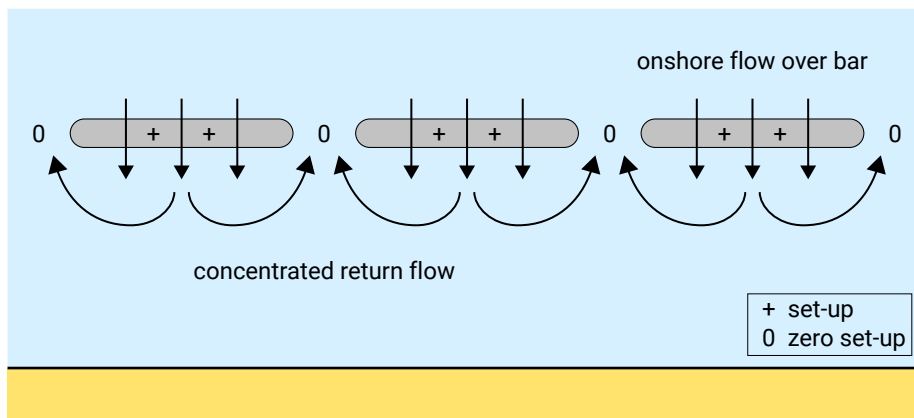
Figure 5.49: Rip currents in case of submerged breakwaters (or an interrupted bar system).
