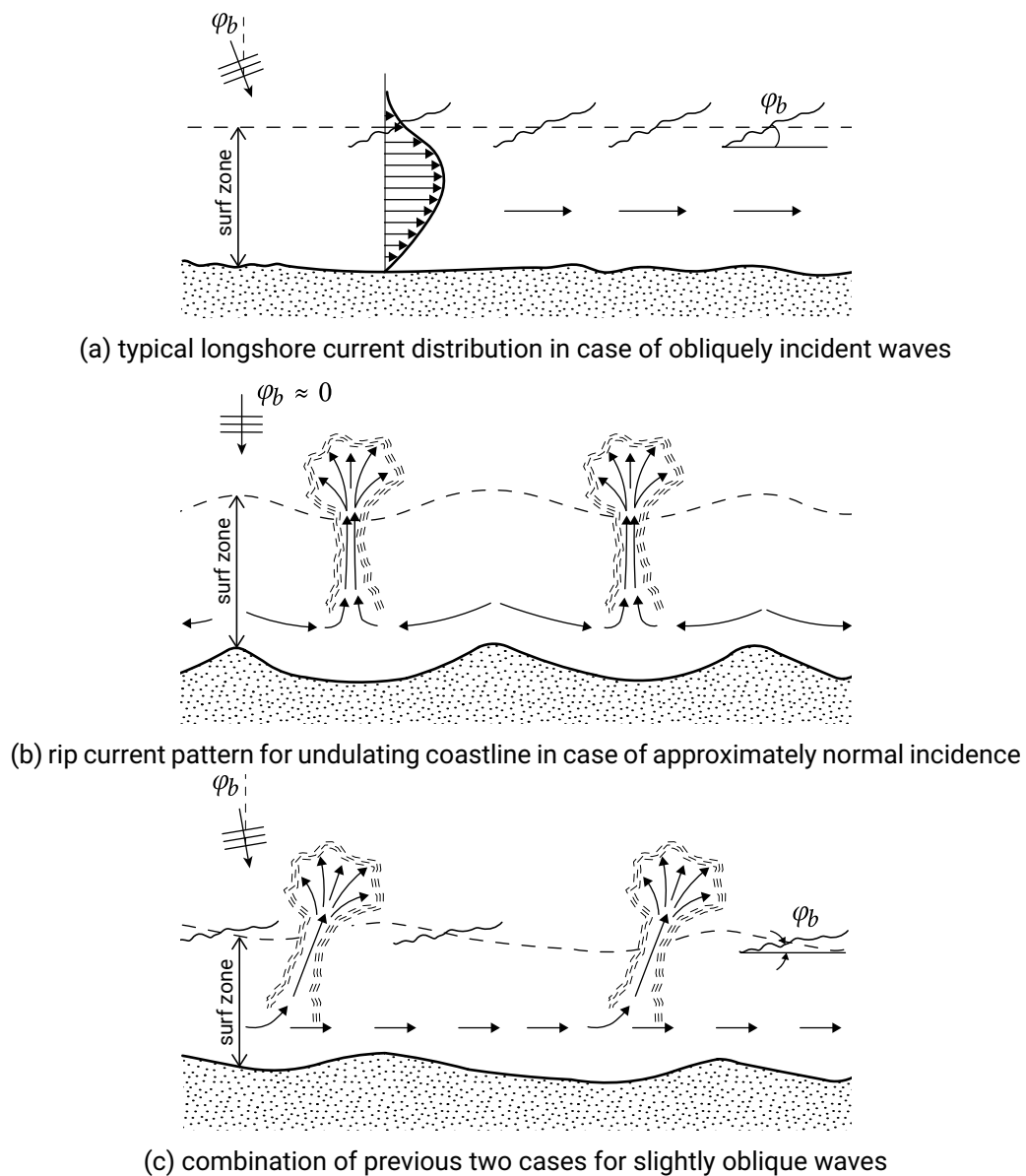
Figure 5.47: Nearshore circulation patterns for different angles of wave incidence \varphi_b .
