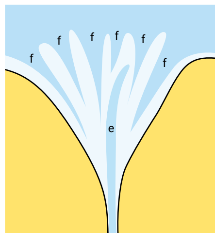
Figure 9.8: Sketch of ebb (e) and flood channels (f) in a wide estuary (for example, the Thames or Wash). Meander action may bring the ebb channel in connection with any of the flood channels (after Van Veen et al., 2005).
