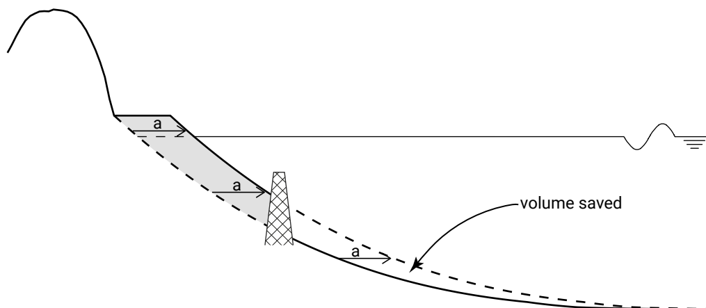
Figure 10.38: Cross-shore profiles in the case of large-scale land reclamation. The shaded volume is saved if a 'perched' beach supported by a submerged breakwater is chosen.
