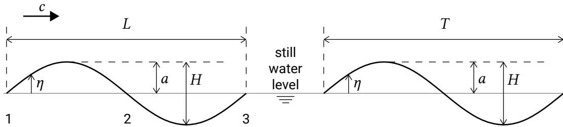
Figure 3.1: Simple representation of a wave. Left: the spatial variation is measured along the direction of wave propagation at a single moment in time. Right: the temporal variation in water level \eta is measured over a certain time period at a single location (at location 2 and directly following the recording of the spatial variation). A similar signal measured simultaneously at location 1 (or 3) will have opposite sign.
