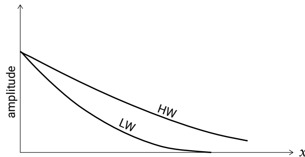
Figure 5.67: Amplitudes of HW and LW for tidal propagation along a basin ( x -axis). In this case, HW is damped less by friction than LW, and, consequently, HW propagates faster than LW. This is particularly true if, due to river discharge, the flow velocity at ebb is much higher than at flood.
