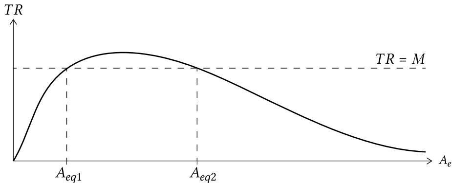
Figure 9.23: Equilibrium cross-sectional areas (Eqs. 9.11 and 9.12).
