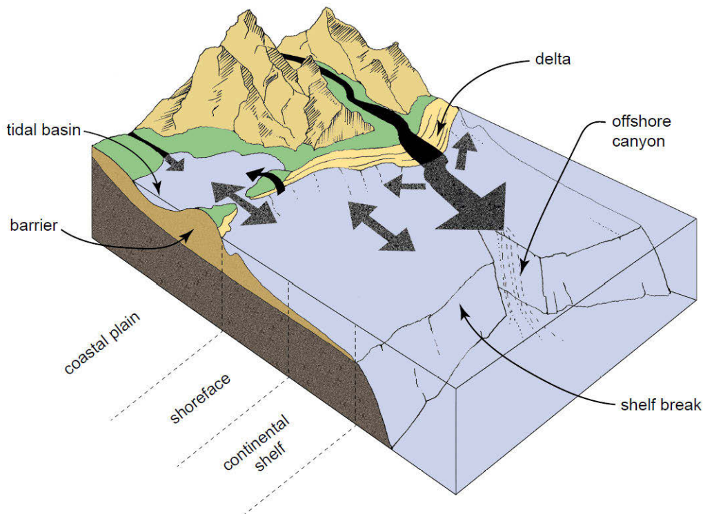
Figure 7.4: The shoreface is the zone between the shore and the continental shelf. On larger timescales the entire shoreface is influenced by wave action and morphodynamically active. The shelf extends to the shelf break.
