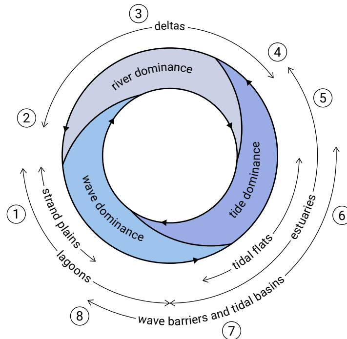
Figure 2.41: The relative influence of fluvial, wave and tidal processes influences the shape of coastal features. The numbers in the figure correspond to the typical morphologies of Fig. 2.42.
