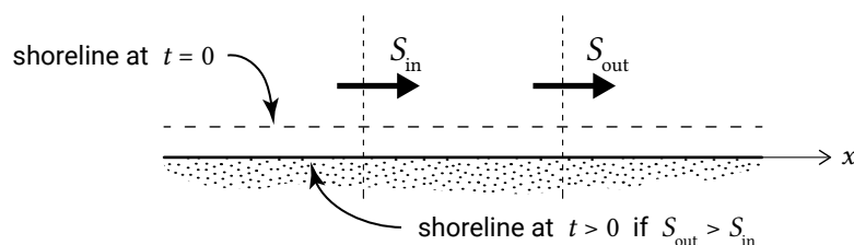
Figure 8.6: Longshore transport continuity.
