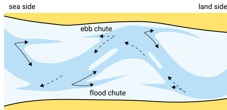
Figure 9.24: Meandering tidal channel with ebb and flood chutes (in Dutch: ebscharen and vloed-scharen ).
