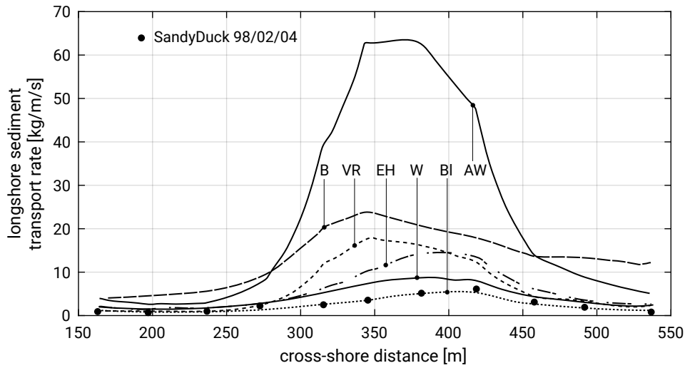
Figure 8.2: Comparison between calculated and measured cross-shore distribution of longshore sediment transport rate for one run of the SandyDuck experiment (98/02/04). Adapted from Bayram et al. (2001). The letters indicate different models, amongst them B: Bijker (Eq. 6.27), BI: Bailard-Inman (Sect. 6.7.2), VR: Van Rijn (Eq. 6.33 for suspended load plus separate bed load formula).
