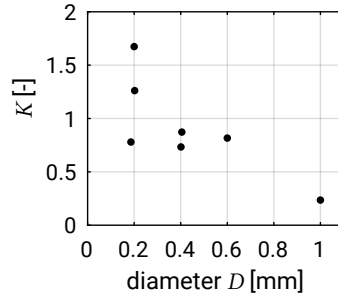
Figure 8.3: Variation in K with grain size (denoted by D ) according to Dean et al. (1982). Note that the dependency of K on D is convincing only for larger grain sizes.
