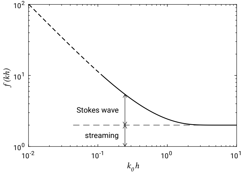
Figure 7.22: The term f(kh) = 2 + (\sinh kh)^{-2} (see Eq. 7.29), plotted as a function of the nondimensional depth k_0 h , where k_0 = \omega^2/g is the deep-water wavenumber.
