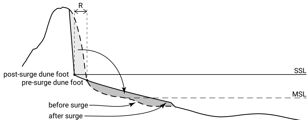
Figure 10.5: Dune erosion during a severe storm surge redistributes sediments in the cross-shore direction. There is no loss of sediment in the alongshore direction and hence the sediment will return under moderate conditions, through the combined action of small waves (under water) and onshore wind (on the beach).
