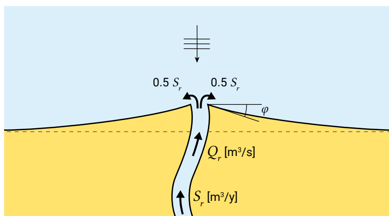
Figure 8.30: Development of deltaic coastline with waves that are normally incident to the original coastline and without tidal influence. The river discharge is Q_r and the sediment discharge is S_r . The angle \phi is determined by the sediment discharge and wave conditions.
