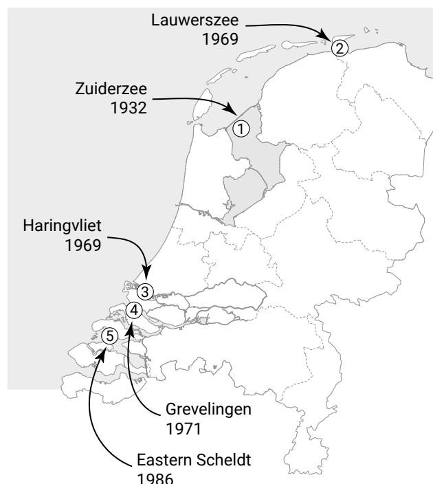
Figure 9.2: Closure of tidal basins in the Dutch coastal system, with the estuaries of the southwestern delta area and the northern Wadden Sea. The Western Scheldt (not numbered) is located to the south of the Eastern Scheldt.
