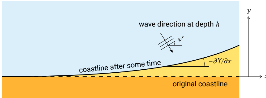
Figure 8.9: Shoreline position Y in original position and after some time. In this figure \varphi is the original angle of wave incidence. After the change in shoreline orientation, this angle has been reduced with \partial Y / \partial x .
