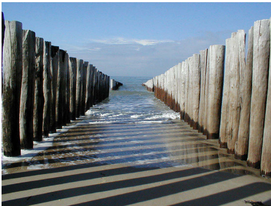
Figure 10.14: A row of piles serving as a groyne at the Zeeland coast in March 2004. This is only one of many types of groynes. Photo by Ad Reniers (see Credits on page 575).
