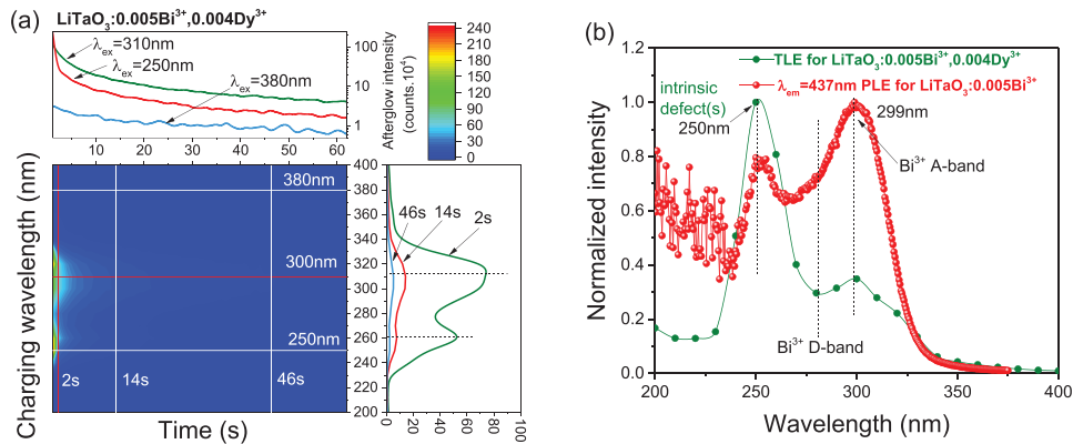
Figure 7. a) 2D contour plot for room temperature (298 K) isothermal decay curves for LiTaO 3 :0.005Bi 3+ , 0.004Dy 3+ as a function of charging wavelength in the range from 200 to 400 nm. The Dy 3+ emission at 580 nm was monitored during this measurement. b) A comparison of the photoluminescence excitation spectrum of LiTaO 3 :0.005Bi 3+ ( \lambda_{em} = 437 nm) and the thermoluminescence excitation (TLE) curves of LiTaO 3 :0.005Bi 3+ , 0.004Dy 3+ .
