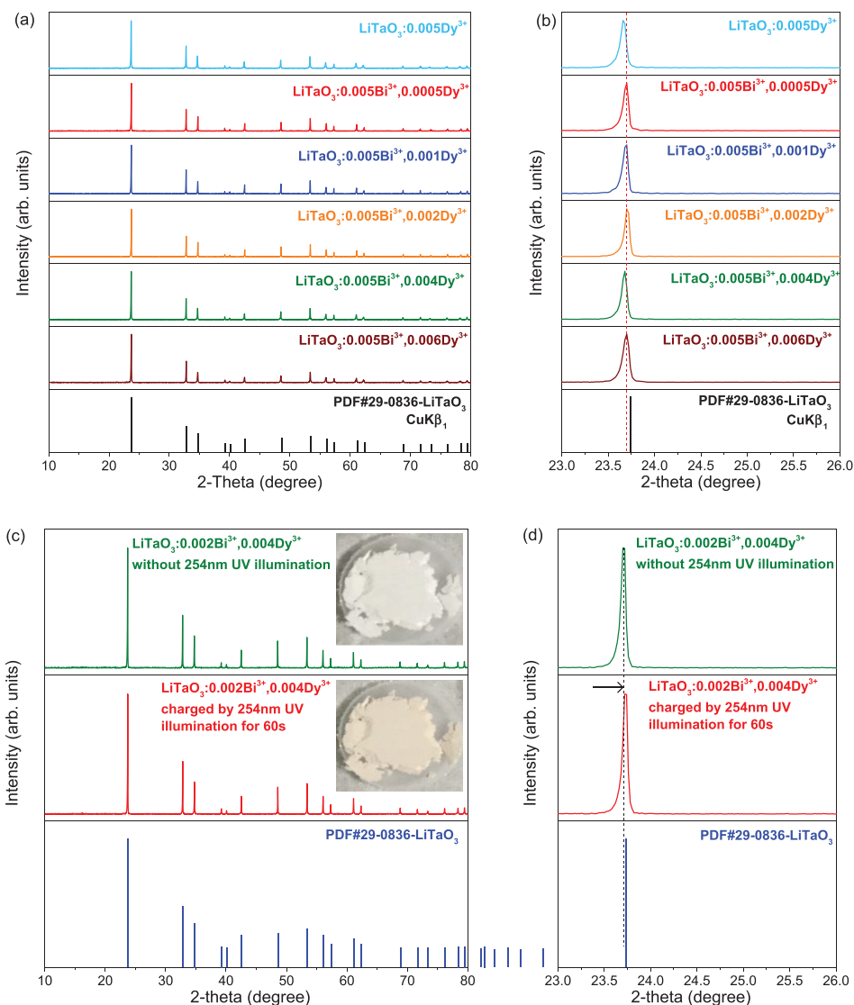
Figure 2. a) XRD patterns from 10° to 80° and b) detailed XRD patterns in the range from 23° to 26° for Bi 3+ and/or Dy 3+ doped LiTaO 3 . c) XRD patterns and d) detailed XRD patterns for the prepared LiTaO 3 :0.002Bi 3+ ,0.004Dy 3+ prior to 254 nm UV-light illumination and after 254 nm UV-light illumination. The inset in panel (c) shows the photographs before and after 254 nm UV-light illumination for a duration of 60 s.
