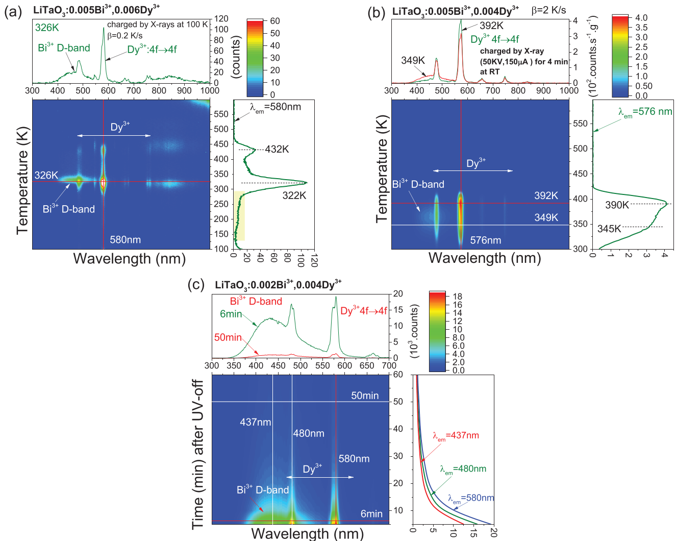
Figure 5. a) The above 100 K TLEM plot measured at \beta = 0.2 \text{ K s}^{-1} for \text{LiTaO}_3:0.005\text{Bi}^{3+}, 0.006\text{Dy}^{3+} after exposure to X-rays at 100 K, b) above-RT TLEM plot measured at \beta = 2 \text{ K s}^{-1} for \text{LiTaO}_3:0.005\text{Bi}^{3+}, 0.004\text{Dy}^{3+} after exposure to X-rays at \approx 298 \text{ K} . c) RT ( \approx 298 \text{ K} ) isothermal decay spectra for \text{LiTaO}_3:0.002\text{Bi}^{3+}, 0.004\text{Dy}^{3+} as a function of time after exposure to 254 nm UV light in the dark.
