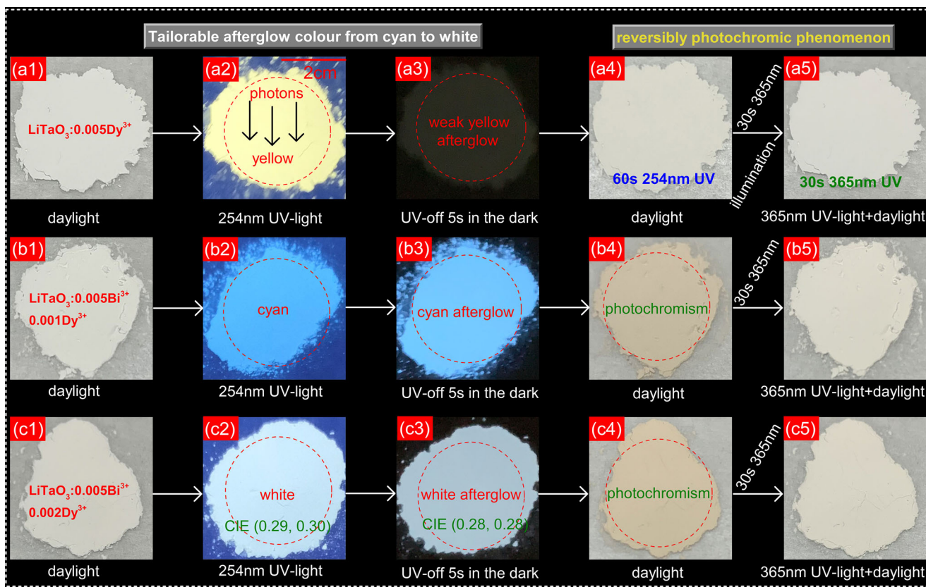
Figure 3. Photographs on rows a), b), and c), pertain to the as-synthesized LiTaO 3 :0.005Dy 3+ , LiTaO 3 :0.005Bi 3+ ,0.001Dy 3+ , and LiTaO 3 :0.005Bi 3+ ,0.002Dy 3+ , respectively, with column 1) the appearance in daylight, column 2) 254 nm excited photoluminescence, column 3) the afterglow, column 4) photochromic color change, and column 5) the phosphor after bleaching.
