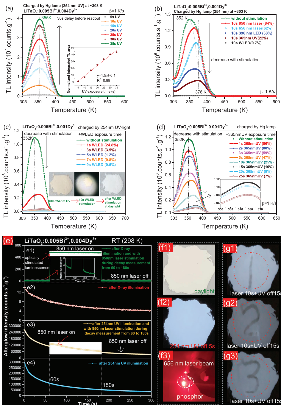
Figure 9. a) TL glow curves at \beta = 1 \text{ K s}^{-1} of \text{LiTaO}_3:0.005\text{Bi}^{3+},0.004\text{Dy}^{3+} after exposure to 254 nm UV light with different duration time. TL glow curves measured at \beta = 1 \text{ K s}^{-1} for \text{LiTaO}_3:0.005\text{Bi}^{3+},0.001\text{Dy}^{3+} after exposure to 254 nm UV-light followed by b) different energy photon stimulation, or with c) WLED and d) 365 nm UV-light stimulation with different duration times. e) RT isothermal decay curves of \text{LiTaO}_3:0.005\text{Bi}^{3+},0.004\text{Dy}^{3+} after exposure to X-rays or 254 nm UV light followed by 850 nm laser stimulation for 120 s from 60 to 180 s. The inset in panel (e1) is the enlarged decay curve. f) and g) Information display of “1, 2, and 3” by utilizing the afterglow and the optically stimulated emission phenomenon in \text{LiTaO}_3:0.005\text{Bi}^{3+},0.004\text{Dy}^{3+} . The inset in panel (a) shows the integrated TL intensity as a function of 254 nm exposure time and the inset in panel (c) shows the color change after WLED stimulation.
