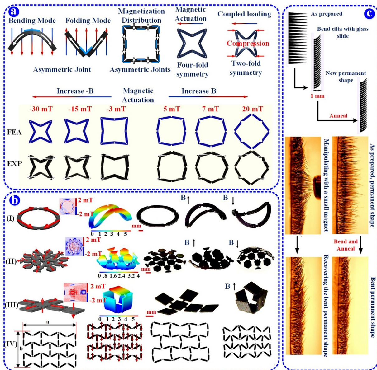
Fig. 14. Applications of MRSM in metamaterials. (a) FE simulation and experiment of the deformation mode of the architected structures under the compression loading at different discrete magnetic field [310]. (b) Reprogrammable 3D reconfigurable structures [4]; I) a four-ligament ring, II) a half-sphere, III) a cubic box and IV) an auxetic metamaterial. (c) a reconfigurable cilia [321] a schematic drawing of the programming of the Irogran magnetic cilia.
