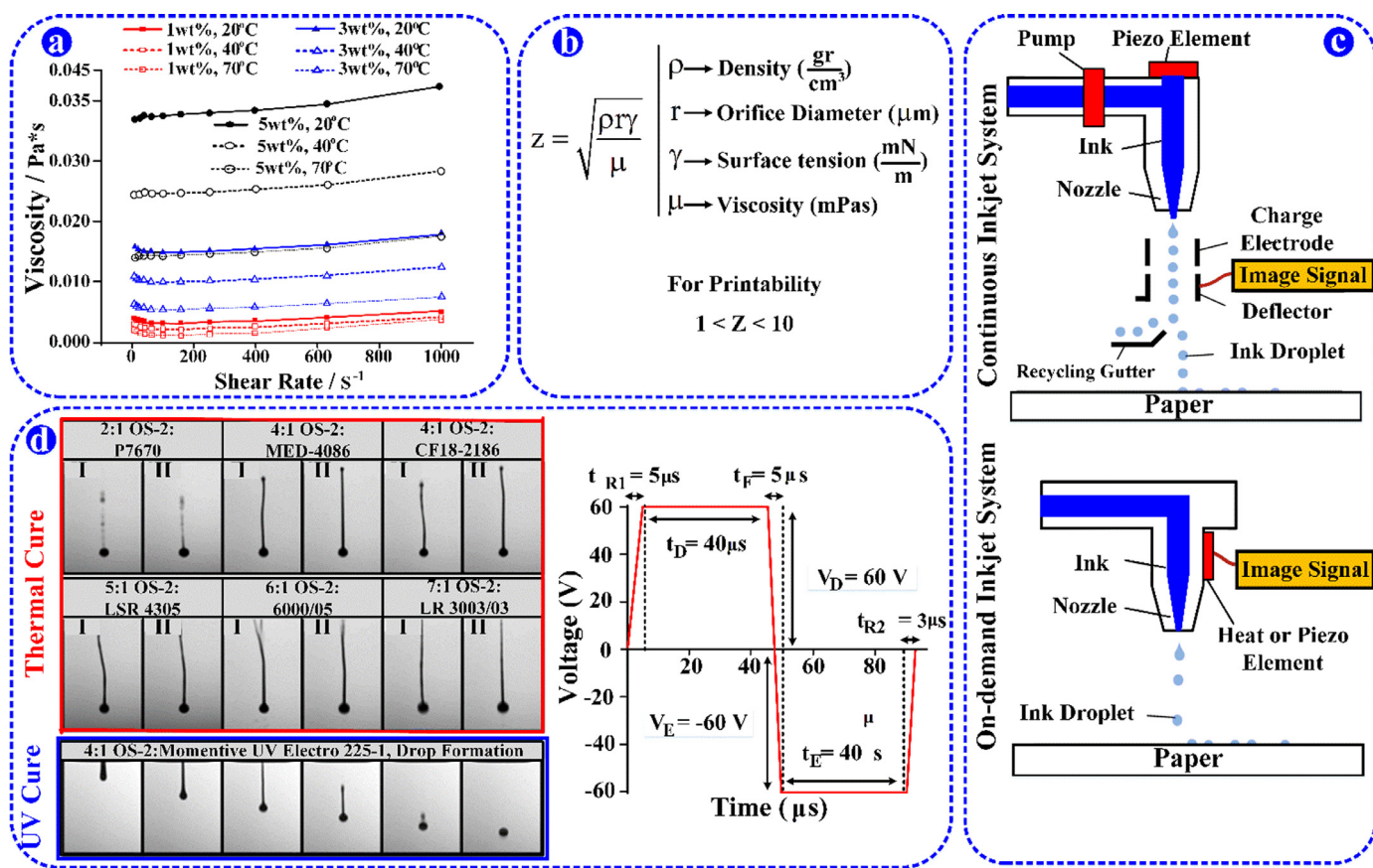
Fig. 3. (a) Example of the physical properties (e.g., viscosity) of the ink in inkjet 3D printing [38]. (b) Important parameters that are necessary to be taken into account for the printability of the ink [38,39]. (c) Schematics showing a continuous inkjet printer and an on-demand inkjet printer [50]. (d) Examples of jetting droplets formed for thermal and UV curable silicone elastomer inks [41].
