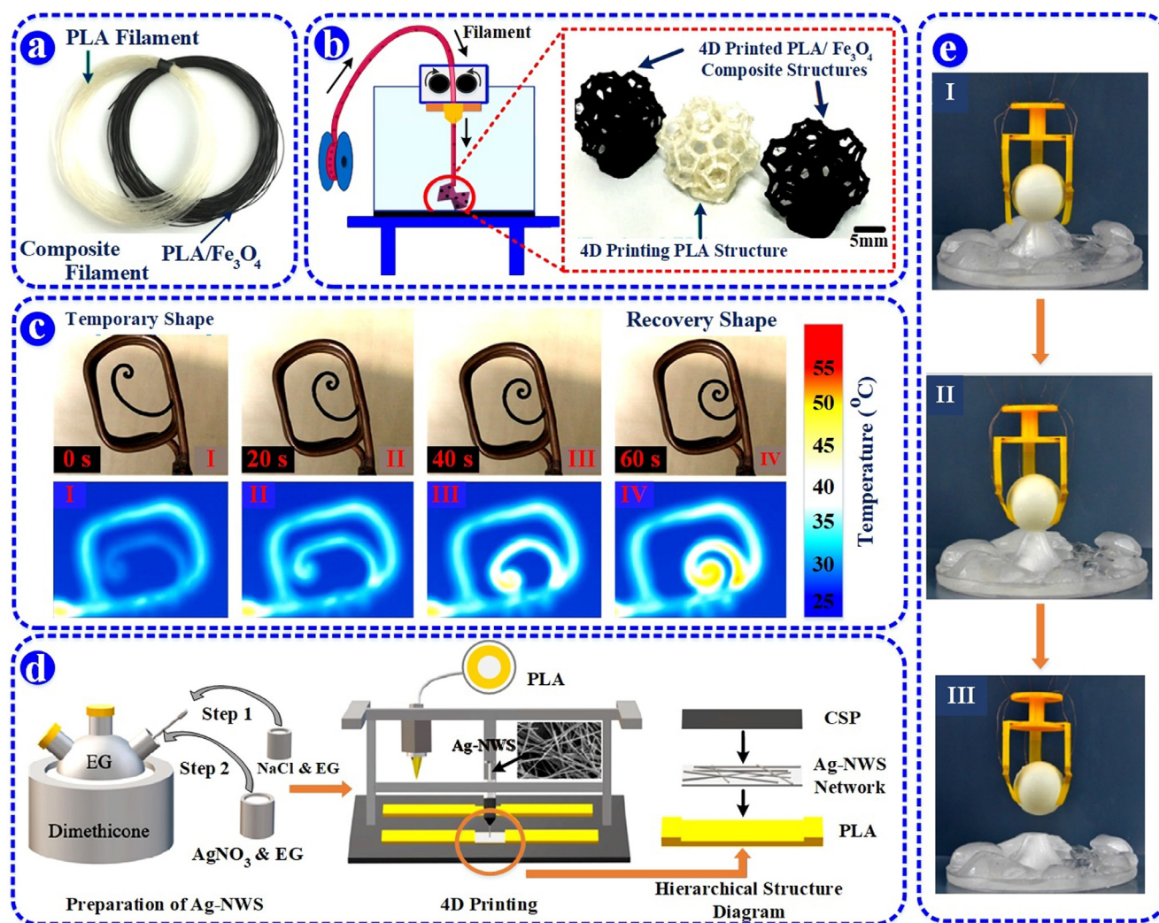
Fig. 4. Examples of the modifications and developments of filaments for 3D/ 4D printing of MERPs using the FDM technique. (a, b and c) FDM for magneto-responsive PLA composite [55]. (d and e) FDM for electro-responsive PLA composite [54].
