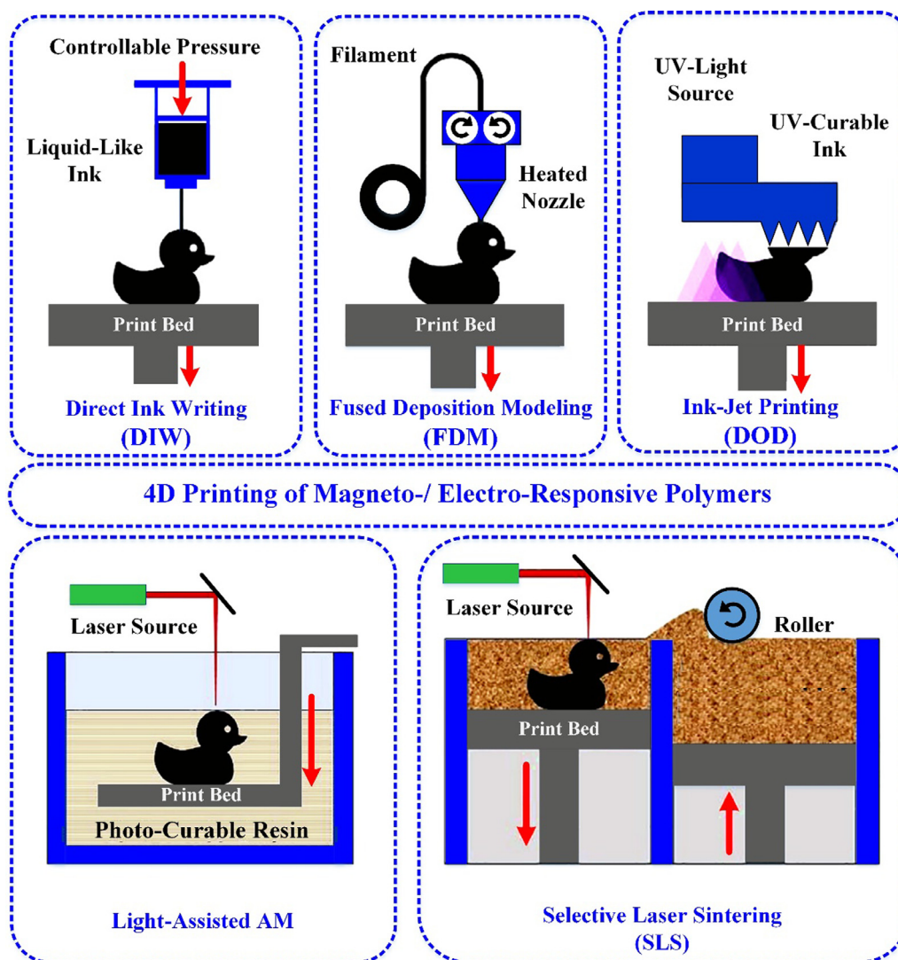
Fig. 1. A schematic summary of the 3D printing techniques used for the development of MERPs. The 3D printing illustrative sub-figures are adapted from [30].
