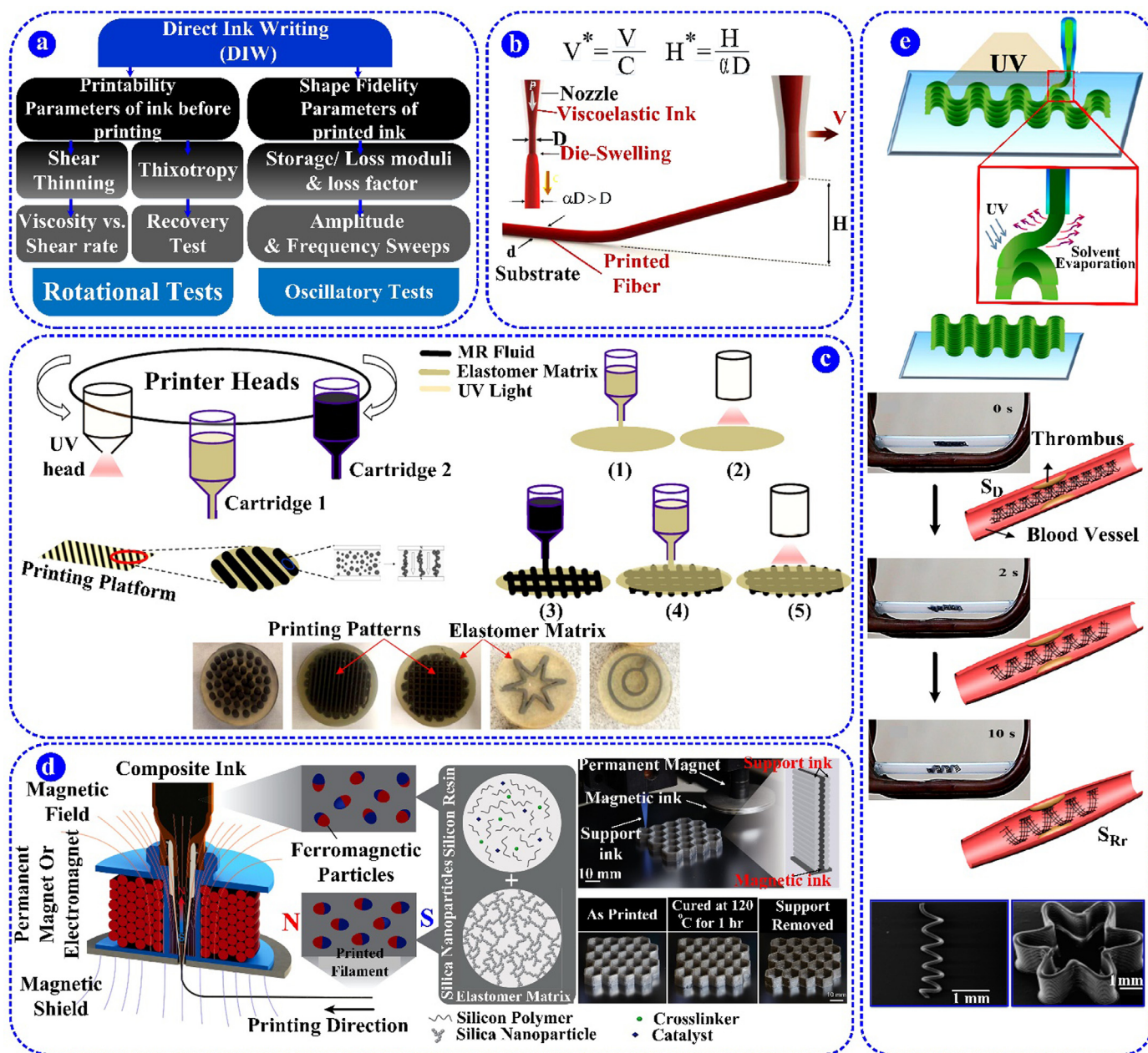
Fig. 2. (a) A summary of the rheological parameters for the development of inks in DIW. (b) Illustration of the optimization of the printing process [33], where V : speed of the nozzle/platform, C : speed of the extruded filament, H : printing height (distance between printing platform and nozzle tip), D : diameter of the extruded filament, \alpha : die swelling ratio, V^* : dimensionless print speed and H^* : dimensionless print height. (c) Schematic illustration of the 3D printing of hybrid MREs using soft magnetic particles and examples of printed patterns [32]. (d) Schematics of the printing process of magnetic domains using hard magnetic particles, the magnetic domains were reoriented by applying a magnetic field generated by a permanent magnet or an electro-magnet placed around the dispensing nozzle and the example of the developed patterns [16]. (e) Schematic of the DIW 3D printing via solvent evaporation of UV cross-linked PLA-based ink and the 3D-printed structures [34].
