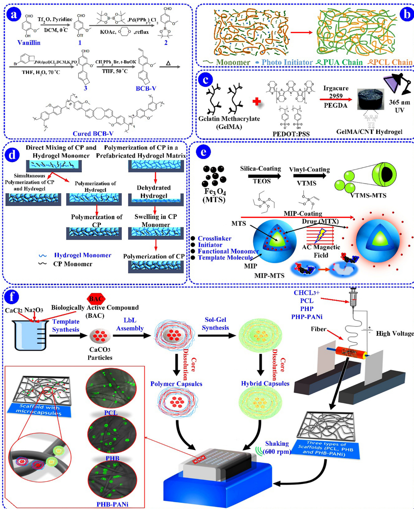
Fig. 7. Some examples of chemical reactions in fabricating MERPs. (a) BCB-V synthesis process in four steps to fabricate a DE. After increasing the temperature, BCB-V becomes a cross-linked network [123]. (b) Schematic of the cross-linking process of poly(urethane acrylate)/ polycaprolactone (PCL) SMP by UV light to fabricate ERPs [88]. (c) Schematic of the polymerization process of a conducting hydrogel [89]. (d) Drawing of a synthesis process of gelatin methacrylate/ CNT conductive hydrogels [130]. (e) Illustration of the preparation of a magneto-responsive drug-release composite system [97]. (f) Schematic of scaffold fabrication processes by the conventional electrospinning setup, synthesis of polymer using layer-by-layer technique and immobilized hybrid capsules [131].
