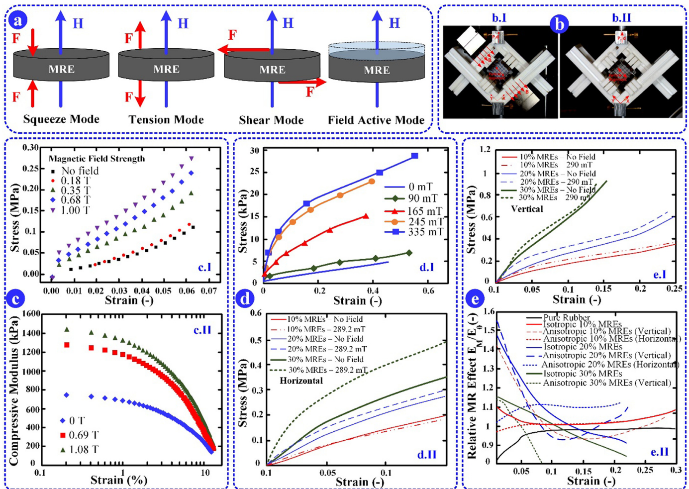
Fig. 8. (a) Experimental samples prepared for magneto-mechanically coupled study in various modes of deformations taken from Bastola and Hossain [73]. (b) a bespoke biaxial test setup made by Harrison and Schubert and Harrison [147]; (I) an anisotropic MRP sample for the pure mechanical test (II) Experimental set up while a magnetic field is applied in a MRP sample in which the field is applied in y-direction parallel to the particle chains of aligned MRPs. (c) Uniaxial compression test results with varying magnetic field as obtained (I) by Kallio [142] and (II) by Gordaninejad et al. [143]. (d) Uniaxial tensile test results under different amounts of magneto-mechanically coupled loads. (I) Stepanov et al. [144] performed tests on isotropic MRPs while (II) Schubert and Harrison [145] used anisotropic MRPs. (e) Pure shear experiments of isotropic and anisotropic magneto-responsive composites conducted by Schubert and Harrison [145]; (I) The influence of magnetic field at the various percentage of fillers, (II) MR effect in both isotropic and anisotropic MRPs.
