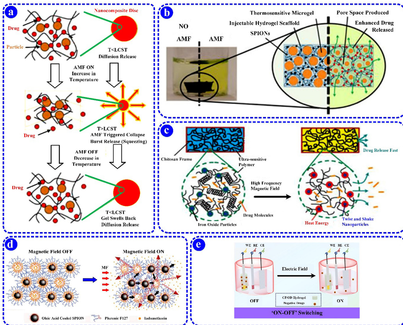
Fig. 12. (a) The schematic of the drug-release of MRPs under an AMF leading to generating an internal heat so that shrinks and squeezes the polymers in such a way that the drug is released [262], (b) Expanding the pore size of a hydrogel scaffold, leading to the increase of drug release [275], (c) Tuning the drug-release based on the heat generated under high-frequency magnetic field [276]. (d) The mechanisms of drug-release based on the on-off magnetic field, resulting in the movement of magnetic particles and therefore squeezes the polymer structure [260]. (e) The mechanisms of drug release in ERPs; the electric field changes pH, resulting in the destruction of hydrogen binding of polymers and eventually the drug release is enhanced [269].
