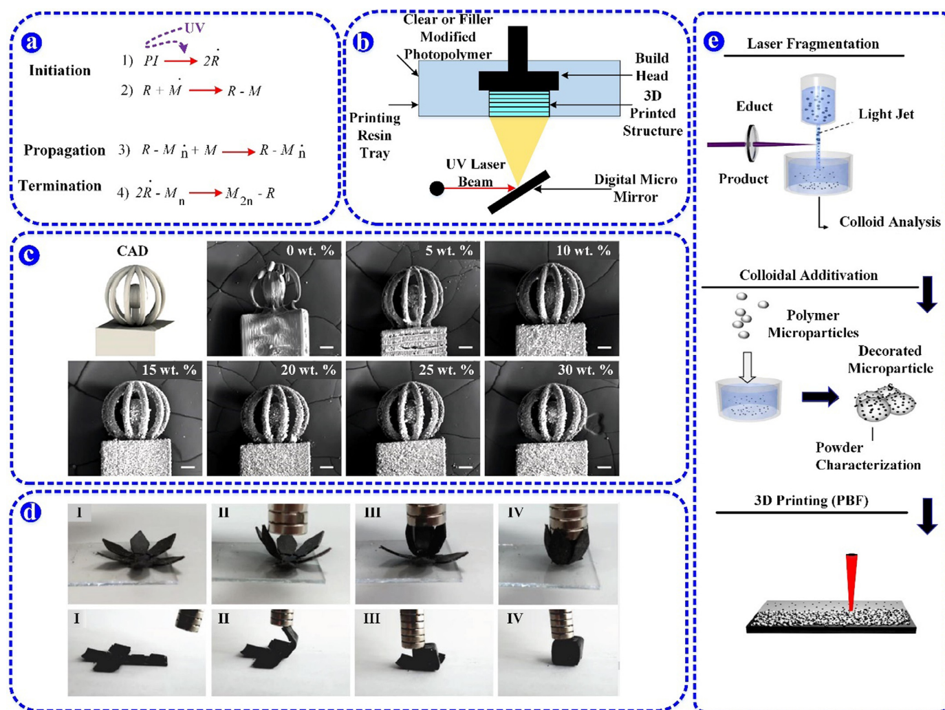
Fig. 5. (a) DLP photopolymerization reaction mechanism [60]. (b) Illustration of DLP 3D printing technique [61]. (c) CAD design of hollow spheres and corresponding 3D-printed samples using magnetic resin via DLP technique [54]. (d) DLP 3D-printed MREs, 3D-printed flower and 2D structure composed of flexible and rigid elements able to create a 3D cube when exposed to a magnetic field [62]. (e) Method to blend NPs of IOs into polyamide for nanocomposite powder development for SLS 3D printing [63].
