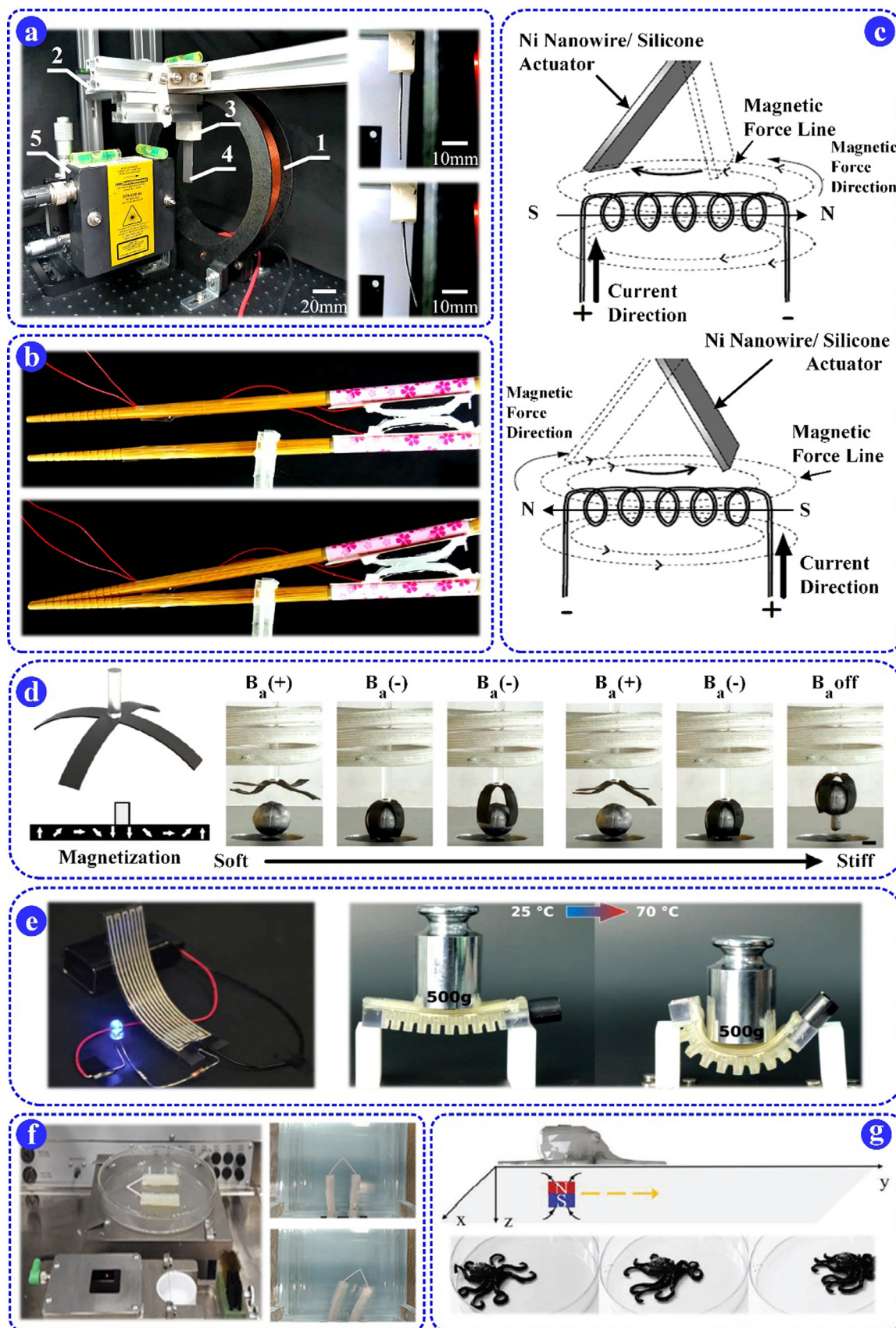
Fig. 16. (a) The MRE soft actuator set up and actuation sequence with application of a magnetic field, 1. Solenoid 2. Structure 3. Sample holder 4. MRE actuator 5. Laser displacement sensor [340]. (b) Chopstick-shape DE soft robot [358]. (c) The EMRE soft actuator under different magnetic fields [376]. (d) a shape locking magnetic SMP with (left) and without (right) locking mechanisms [3]. (e) The printed joule heating circuit of the electric SMP soft gripper (left) and its application in temperature-dependent stiffness variable [389]. (f) 4D-printed electro-responsive hydrogel soft parallel robot and its actuation states [381]. (g) 4D-printed magneto-responsive octopus hydrogel soft robot [36].
