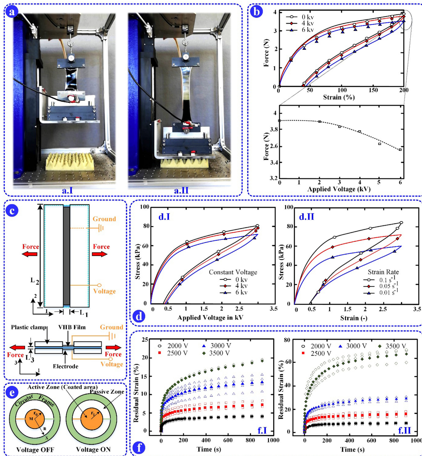
Fig. 9. (a) a bespoke experimental setup for uniaxial tests prepared by Mehnert et al. [157]; (I) an undeformed coated sample (II) Deformed sample under an electro-mechanically load. (b) Stress-strain cycles at different voltages, and the influence of electric voltage on the thickness direction, i.e., release of stress in the vertical direction [157]. (c) a pure shear experimental setup advocated by Chen et al. [165], top view of a coated sample maintaining pure shear geometry and a cross-sectional view of the sample and clamps. (d) Electro-viscoelastic response of VHB 4910 polymer; (I) Stress-strain response at different voltages (fixed strain rate) (II) The same behaviour with different strain rates [165]. (e) a classical setup for conducting equi-biaxial electro-mechanical tests, a centrally coated sample before the application of electrical voltage, and actuated sample surrounded by a passive zone, taken from Wissler and Mazza [166]. (f) Time and voltage-dependent radial strain for (I) a 300% pre-strain (II) a 400% pre-strain [166].
