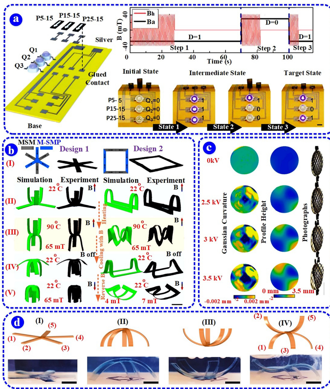
Fig. 15. (a) Application of sequential MRSM with shape locking abilities in digital logic circuits [3]. (b) Computational modelling and experimental results of multi-modal MRSM in a pop-up (design 1) and Asterisk design (design 2) 3D printed by multi-material DIW [69]. (c) ERSM in a DE-based circular sheet; the increasing of negative Gaussian curvature upon increasing applied voltage in a DE [296]. (d) ERSM in electro-responsive hydrogel based on the multipolar spatial electric field to mimic the movement of swollen starfish [140].
