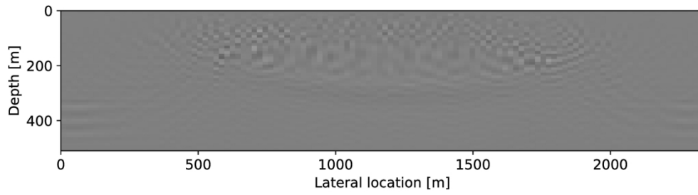
Figure 8d. Imaging up to 40 Hz of the model in Figure \ref{fig:Figure5B_v} with (a) initial and (b) optimized geometries. (c) Amplitude difference between (a) and reference model. (d) Amplitude difference between (b) and reference model. (e) Comparison of target functions.
