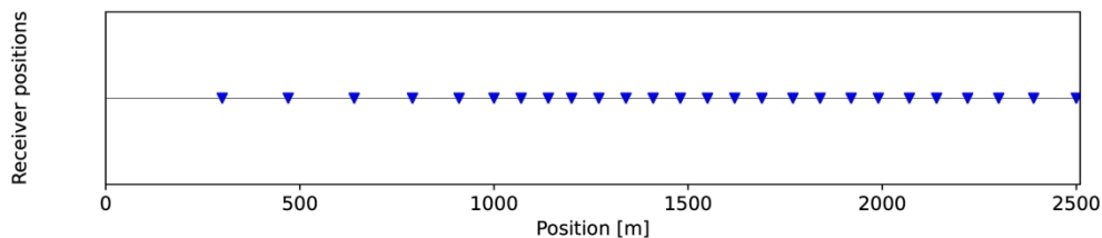
Figure 10d. Optimized receiver geometry for the model in Figure \ref{fig:Figure9_v}. The receivers are located at the surface z=0 m. After optimization, the receivers are re-located towards the right hand side of the model. (a) Initial receiver geometry, (b) initial receiver density, (c) optimized receiver density, (d) optimized receiver geometry.
