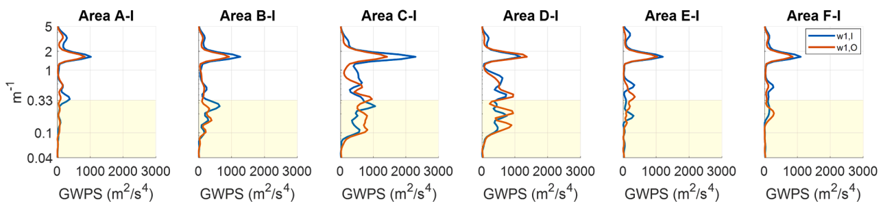
Fig. 15. GWPS of the ABA signals measured at different rails for Track I at Bridge 6.
