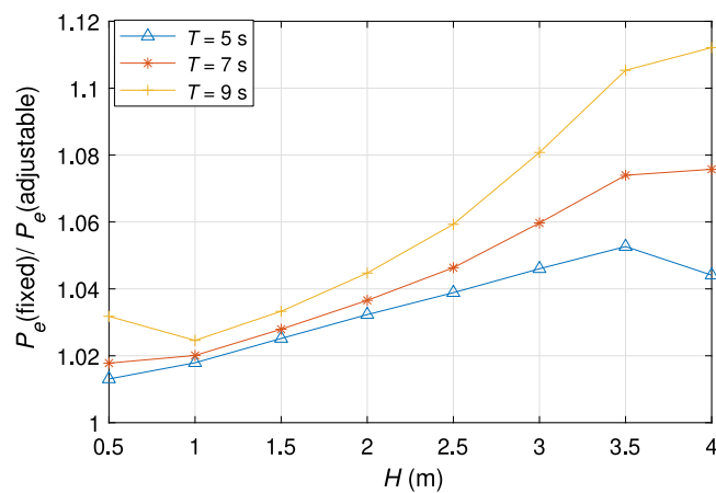
Fig. 13. The average electrical power of the fixed draft WEC with the draft of 3.5 m normalized to that of the adjustable draft WEC with the draft of 3.5 m, and B_{pto} = 30 kNs/m.
