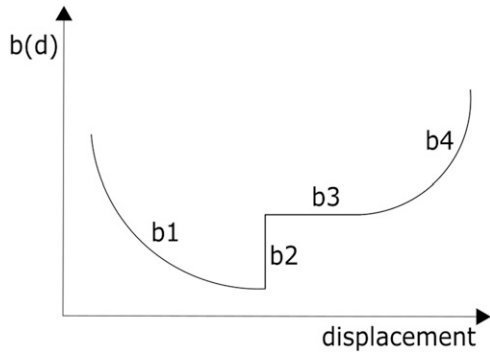
Figure 6. b-value/displacement plot. The possible trends that can be found in actual test are shown.
