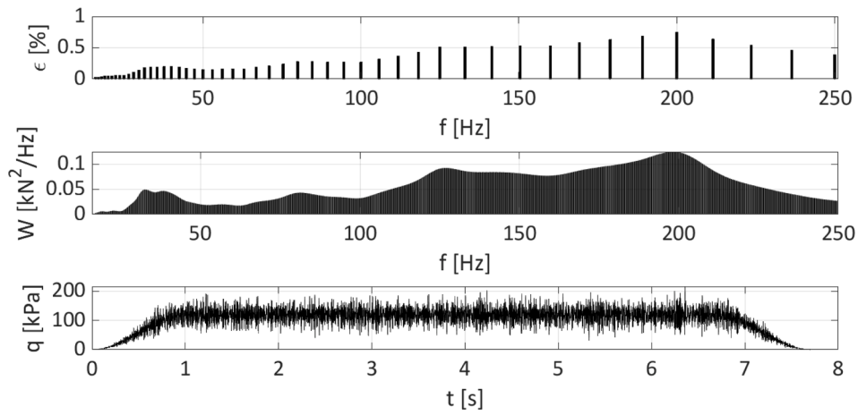
Fig. 9. Non-dimensional dynamic load spectrum [32], estimated power spectral density and time-history of the enforced load (see Fig. 1).
