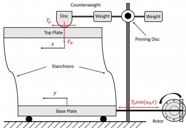
Fig. 4 Schematic diagram of the SDoF single-storey shear frame structure subjected to Coulomb friction. Image adapted from Ref. [43].
