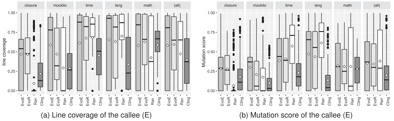
Fig. 8. Effectiveness of T_{CLING} (CLING), T_{EvoE} (EvoE), T_{EvoR} (EvoR), and T_{Ran} (Ran). ( \diamond ) denotes the arithmetic mean and (—) indicates the median.
