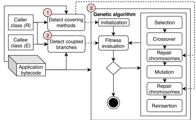
Fig. 2. General overview of CLING.
