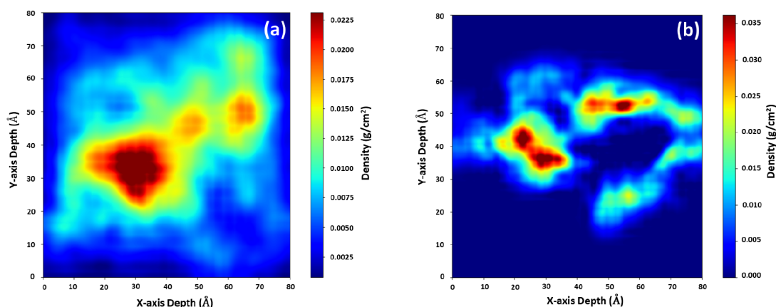
Figure 7. Trajectory density contours for (a) asphaltene in a toluene- [\text{Et}_3\text{NH}]^+[\text{H}_2\text{PO}_4]^- mixture. (b) Asphaltene in a hexane- [\text{Et}_3\text{NH}]^+[\text{H}_2\text{PO}_4]^- mixture.
