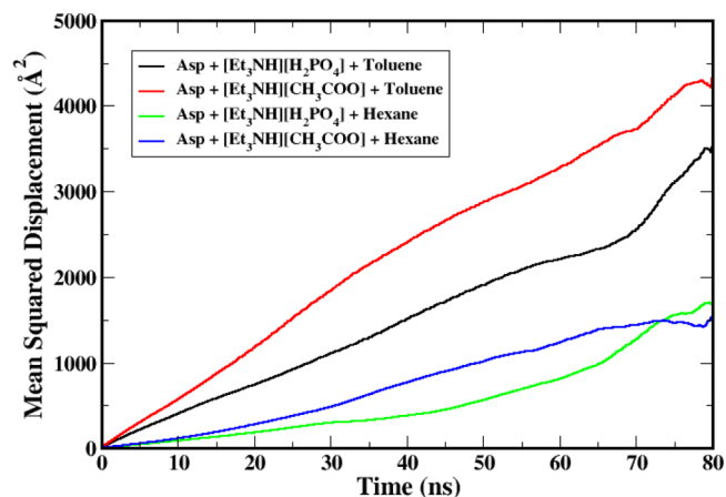
Figure 5. Mean squared displacement of asphaltene in four different asphaltene-IL-toluene/hexane mixtures.
