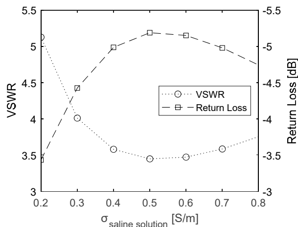
Figure 4. VSWR and Return Loss values calculated as a function of saline solution conductivity.
