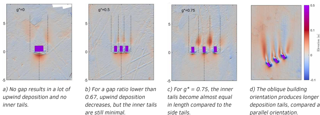
FIG. 3.62 Test results of a scale-model row with varying gap-distances (gap of 0, 1 and 3 times the building's width) and 3 times the buildings width with a 60° wind angle. Measurements (x,y) in meters. Source: Poppema, 2022.
