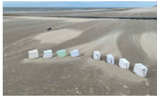
FIG. 3.71 (right) Field test of a V-shaped scaled row house configuration on an open beach plain in Vlieland (2020), combining wind convergence and oblique placement to lengthen tails and guide sediment to the back as an artificial blowout. Image by the author.
