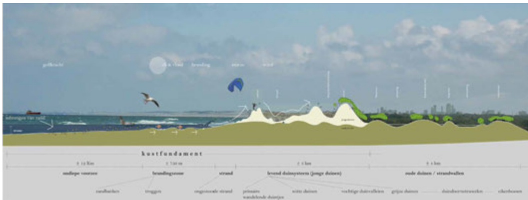
FIG. 2.15 Stages of dune formation. Source: Studio Coastal Quality TU Delft / Paridon & De Groot 2011.
