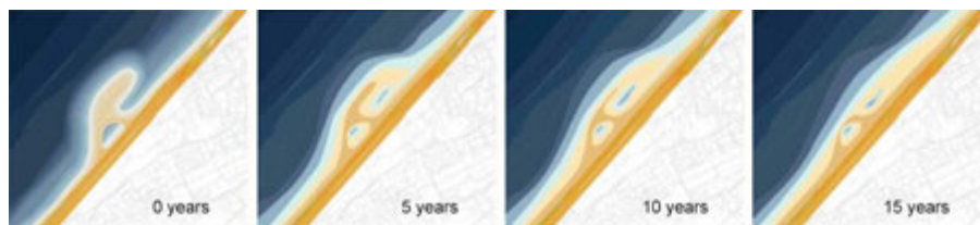
FIG. 4.47 Predicted progress of the Sand Motor. Source: www.dezandmotor.nl .
