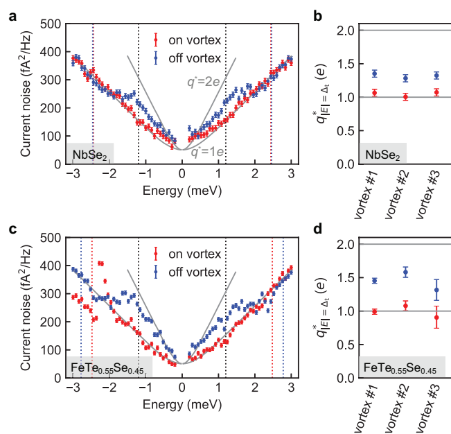
Fig. 4 | Local noise spectroscopy on and off vortices in \text{NbSe}_2 and \text{FeTe}_{0.55}\text{Se}_{0.45} . a, c Current noise spectra in the tunnel junction (with a resistance R_j = 2.5\text{ MOhm} ) taken on (red) and off (blue) the vortex shown in Fig. 2a for \text{NbSe}_2 and Fig. 3a for \text{FeTe}_{0.55}\text{Se}_{0.45} , respectively. The locations of these spectra are marked by the crosses in Figs. 2a and 3a with the same colors. Gray curves are the expected noise from Eq. 2 with an effective charge q^* of 1e and 2e at T = 2.3\text{ K} . The dashed lines in a and c are replicated from Figs. 2b and 3b, respectively, serving as guides for the coherence peaks (red and blue) and the bound states (gray). The error bars are determined by the fluctuation of the current noise in time before each experiment, yielding a standard deviation of 9.25 and 6.77\text{ fA}^2/\text{Hz} for a and c , respectively. b, d Effective charge q^* derived by numerically solving Eq. 2 at the energy E = \pm\Delta_t on (red) and off (blue) vortex for three different vortices in \text{NbSe}_2 and \text{FeTe}_{0.55}\text{Se}_{0.45} , respectively. The error bars are determined by the standard deviation of the extracted q^* (Supplementary Figs. 3–5) in the energy ranges (\Delta_t \pm 0.1\text{ meV}) and -(\Delta_t \pm 0.1\text{ meV}) .
