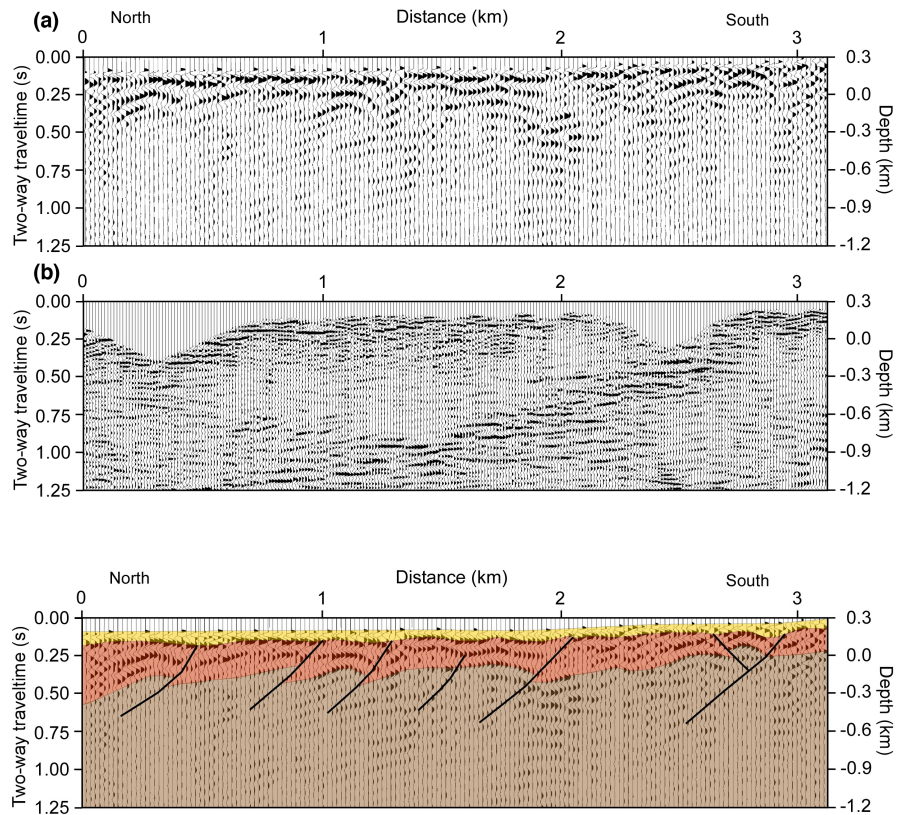
FIGURE 10 Interpreted version of the passive seismic section from Figure 9a ; Middle Miocene -yellow, Paleogene - dark red and Basement - brown, possible Miocene faults - black lines.
