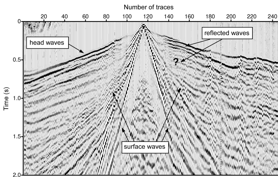
FIGURE 8 Active-source seismic reflection record with shot point near receiver number 115. Trace spacing of 12.5 m. Band-pass frequency filter (2–32 Hz) applied for better display. Static corrections have not been applied.
