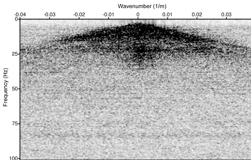
FIGURE 6 The (f, k)-amplitude spectrum of the noise panel from Figure 5.
