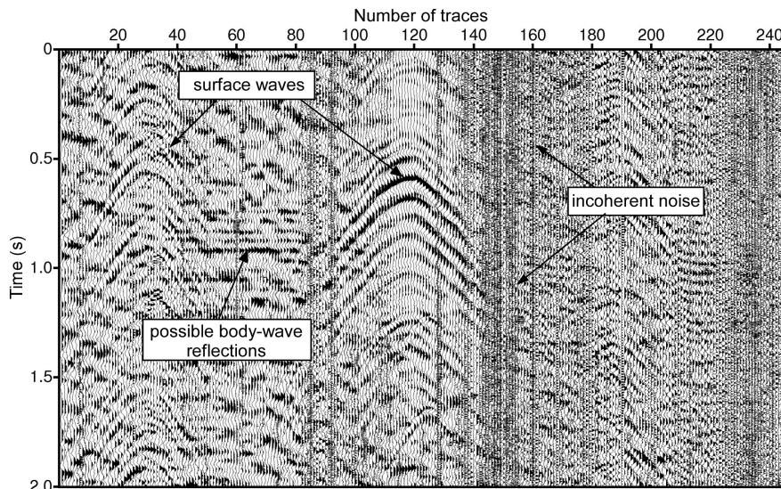
FIGURE 5 Noise panel displayed in the time domain showing possible body-wave reflections, surface waves generated by noise sources and incoherent noise.
