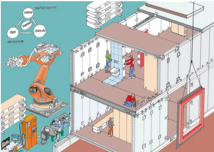
Fig. 17.7 Dismantlable building
