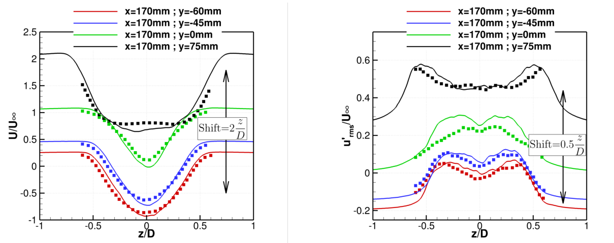
Fig. 14 Mean and RMS velocity profiles at x = 170\text{ mm} ( x/D = 1.13 ) for the solid fairing configuration. Left: mean streamwise velocity u ; Right: streamwise RMS velocity fluctuations u' . Symbols: experiment; solid lines: ZDES simulation.
