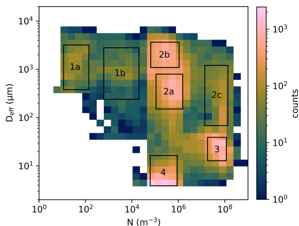
Figure 6. N versus D_{\text{eff}} for 1 Hz low-level particle data over sea ice and the open ocean (< 500 m) from the AFLUX and MOSAiC-ACA campaign combined, color coded by their occurrence. Regimes with increased occurrence frequency are marked with a rectangle. Associated cloud particles: 1 – ice, 2 – mixed-phase, 3 – liquid, and 4 – aerosol particles.
