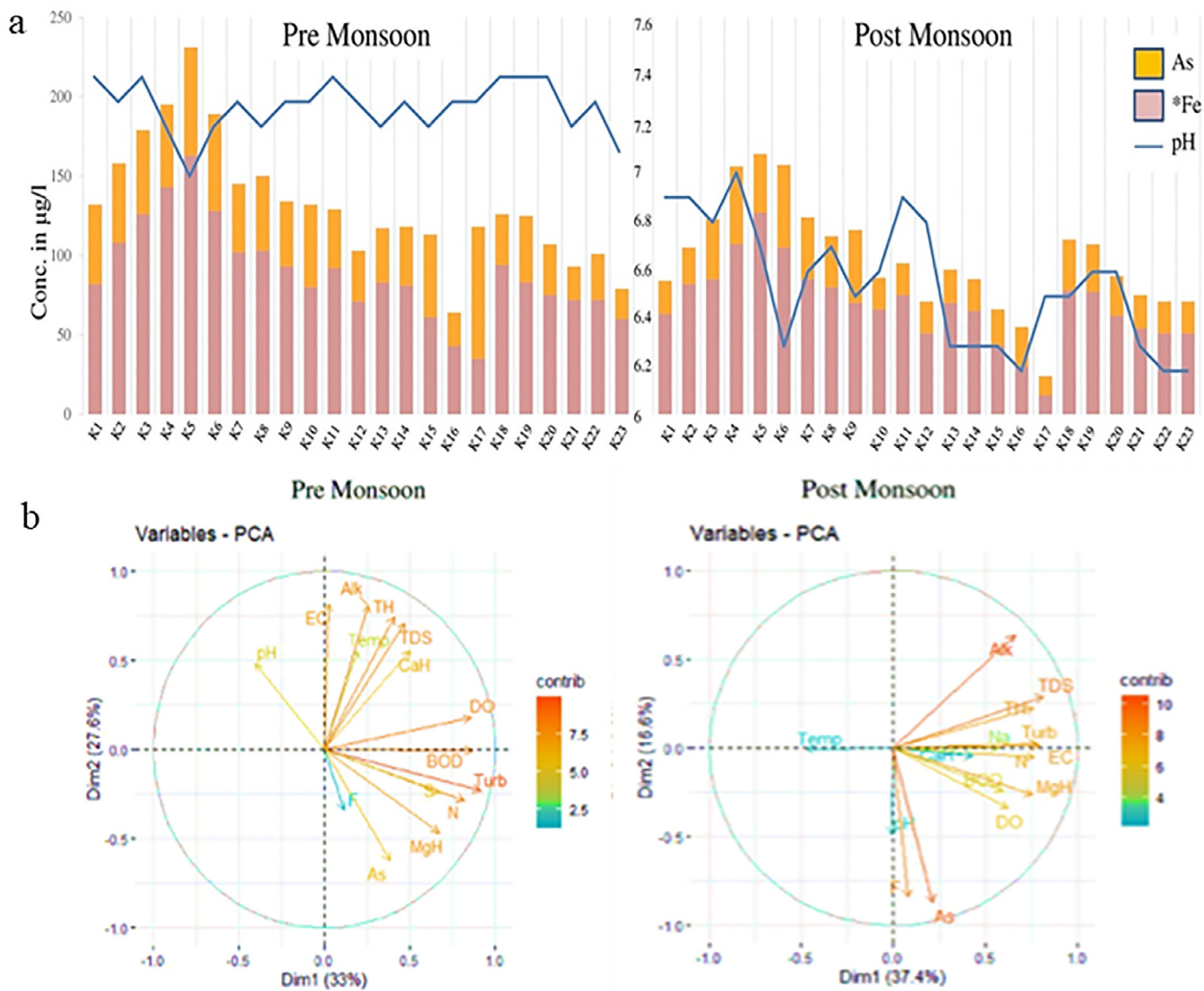
Fig. 3. (a) Alteration in As and Fe concentration of the 23 groundwater samples collected during pre-monsoon and post monsoon seasons along with change in pH [ ^{10} Concentration of Fe is 10X], (b) The PCA of the correlation between physicochemical parameters and elemental fluxes during pre and post monsoon sampling seasons. Plots highlight the association of toxic elements with geo-chemical parameters such as pH.
