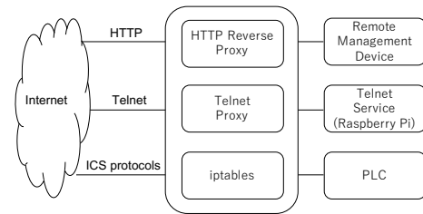
Fig. 5. Honeypot architecture
