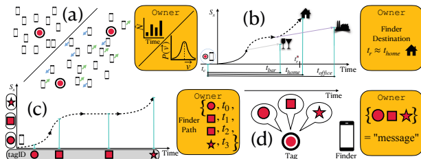
Fig. 4: Overview of alternative uses for the Apple FindMy service. (a) Crowd monitoring. (b) Remote destination inference. (c) Path reconstruction. (d) Covert communication.
