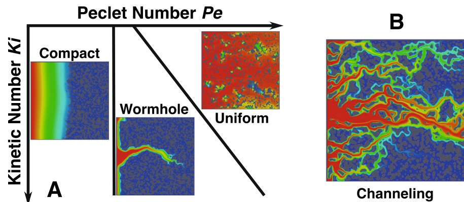
Figure 1. (A) Schematic depiction of dissolution regimes in the Péclet number—kinetic number space. (B) This paper modifies this traditional conceptual model by adding the channeling regime.
