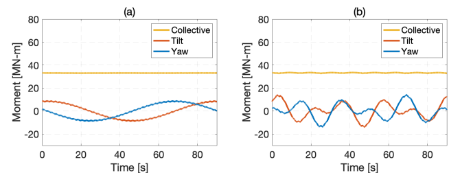
Fig. 3. Moment signals in the fixed frame for simulation cases of (a) SS (b) MS. The collective, tilt, and yaw moments are represented by the yellow, orange and blue line, respectively.
