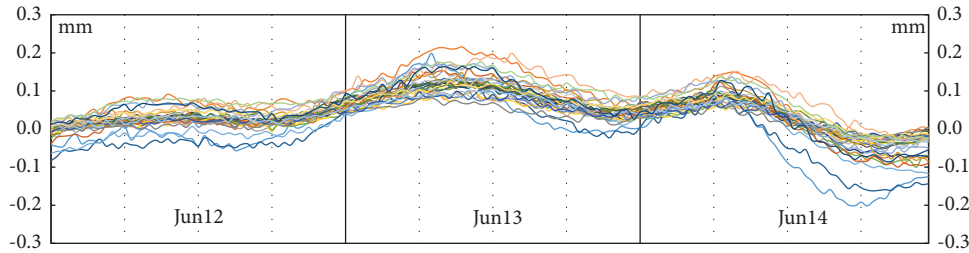
FIGURE 16: Measured joint opening.
