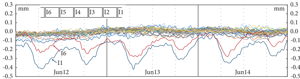
FIGURE 17: Measured joint uneven settlement (values for I6 plotted inverted).
