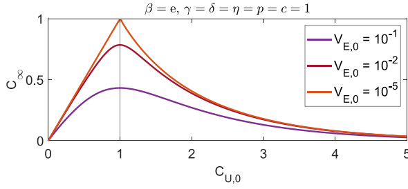
Fig. 2. Asymptotic value C_\infty of C_U as a function of the initial condition C_{U,0} , when \beta = e and all other parameters are set to 1, resulting in \mathcal{C}_U^* = 1 . All the statements in Proposition 3 hold for V_{E,0} = 10^{-5} . As the initial amount of external virus V_{E,0} is increased, C_\infty(C_{U,0}) < \mathcal{C}_U^* , but all statements except for (ii) still hold.
