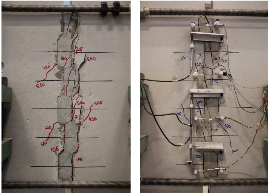
Figure D.3: Specimen 2-4: Residual shear load V_{F,r} = 340 kN
