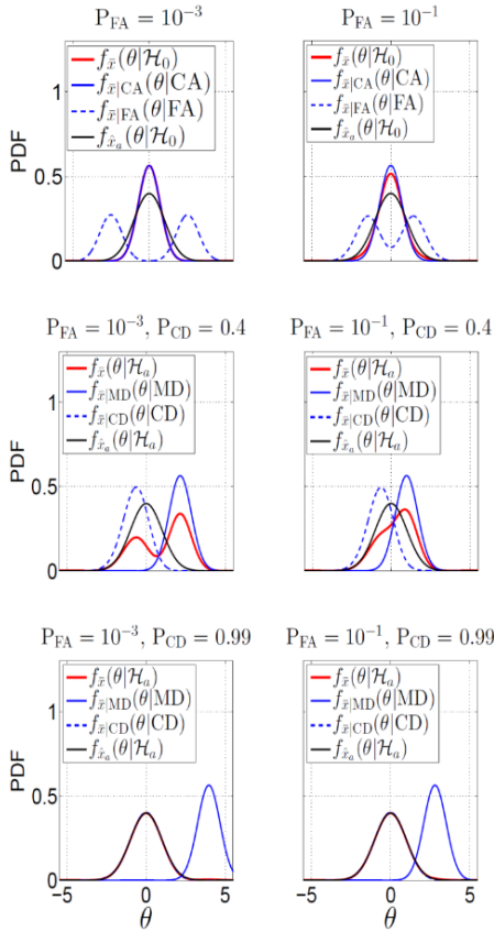
Figure 2. Illustration of the DIA-estimator PDF [top] under null hypothesis H_0 and [middle and bottom] under alternative hypothesis H_a . The contributing parameters are set as \sigma_{x_0}^2 = 0.5\text{m}^2 , \sigma_r^2 = 2\text{m}^2 , L_a = 0.5 . Panels, from left to right, correspond to P_{FA} = 10^{-3} and P_{FA} = 10^{-1} . Panels in the middle and at the bottom correspond to resp. P_{CD} = 0.4 and P_{CD} = 0.99 .
