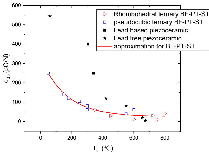
Figure 4. Relationship of piezoelectric properties at room temperature and Curie temperature [9,19].
