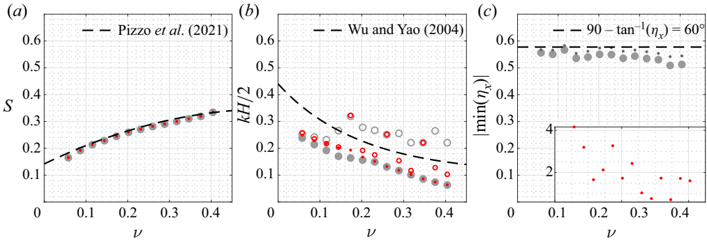
Figure 5. Global and local measures of maximum steepness as a function of bandwidth for the steepest non-breaking (grey markers) and least steep breaking (red dots) wave groups based on constant-steepness spectra. In panel (b) closed markers correspond to steepness measured \pm T_c/2 either side of the time of maximum slope |\min(\eta_x)| , and open markers correspond to maxima observed without this time constraint; in panel (c) the smaller dark grey dots correspond to simulations that were rerun using increased particle resolution at the crest (Configuration B). The inset in panel (c) shows the (much higher) values of maximum slope of breaking wave groups.
