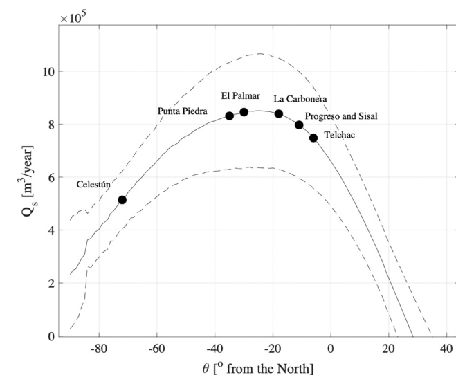
Fig. 4. Net alongshore sediment transport as a function of shoreline orientation. The circles represent selected sites along the study area.
