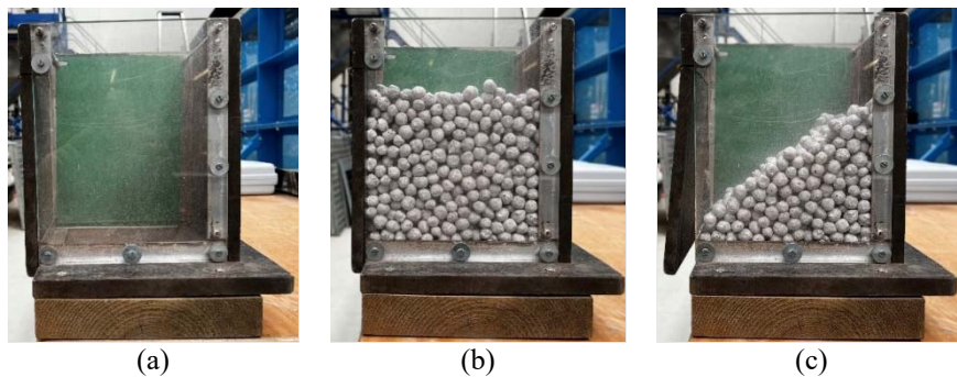
Figure 3 a) Ledge Test Box, b) Filled Ledge Box, and c) the Slope Formed at the End of the Test
