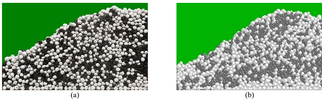
Figure 14 Results of Multi-Component Mixture of Sinter (Black) and Pellets (White) a) Experiments and b) Calibrated DEM Model Output Based on Parameter Set 2 (see Table 6).
