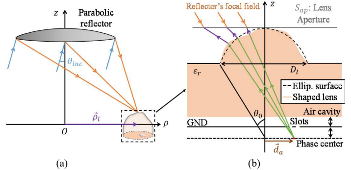
Fig. 1. (a) Schematic representation of the shaped quartz lens coupled to a parabolic reflector which is illuminated by a plane wave with the incident angle of \theta_{inc} . (b) Zoomed-in lens geometry. Green and purple rays represent the antenna primary and lens secondary fields, respectively.
