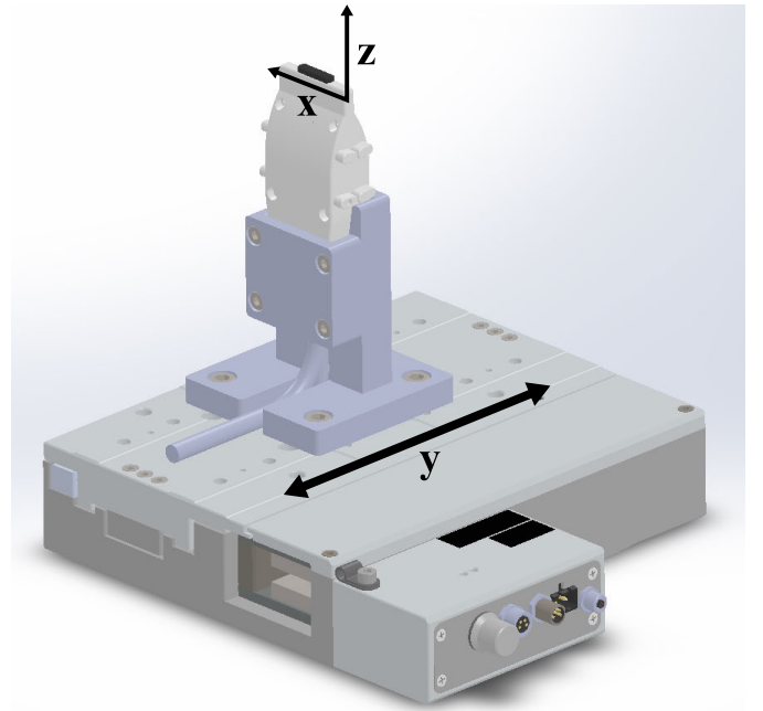
Fig. 2. Schematic of the L22-14v ultrasound transducer attached to a motorized linear stage using a custom probe holder. The y-axis shows the direction of movement of the linear stage, while the x- and z-axis show the imaging plane of the ultrasound transducer.
