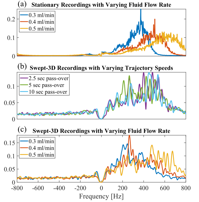
Fig. 9. Doppler spectrum of flow phantom. (a) Doppler spectrum obtained from a stationary recording for three different Doppler flow rates of 0.3, 0.4, and 0.5 ml/min. (b) Swept-3-D Doppler spectrum obtained from three sweep speeds for a constant Doppler flow rate of 0.4 ml/min. (c) Swept-3-D Doppler spectrum obtained for the same Doppler flow rates as used in (a).
