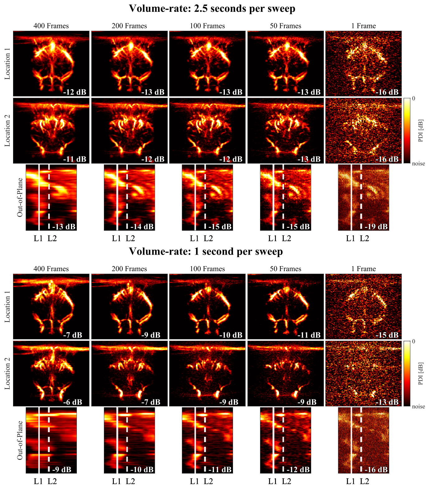
Fig. 10. Averaging of coronal swept-3-D frames over a sweep for two different trajectory speeds. The top three rows contain swept-3-D data from a 2.5 s sweep time, where for each column a PDI was created by averaging over the specified number of frames. This is shown for two locations, as indicated in the out-of-plane images in the third row. This process was repeated for a swept-3-D recording with a sweep time of 1 s in the following three rows.
