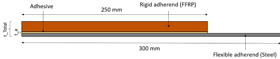
Fig. 4. Scheme of peel sample dimensions.
