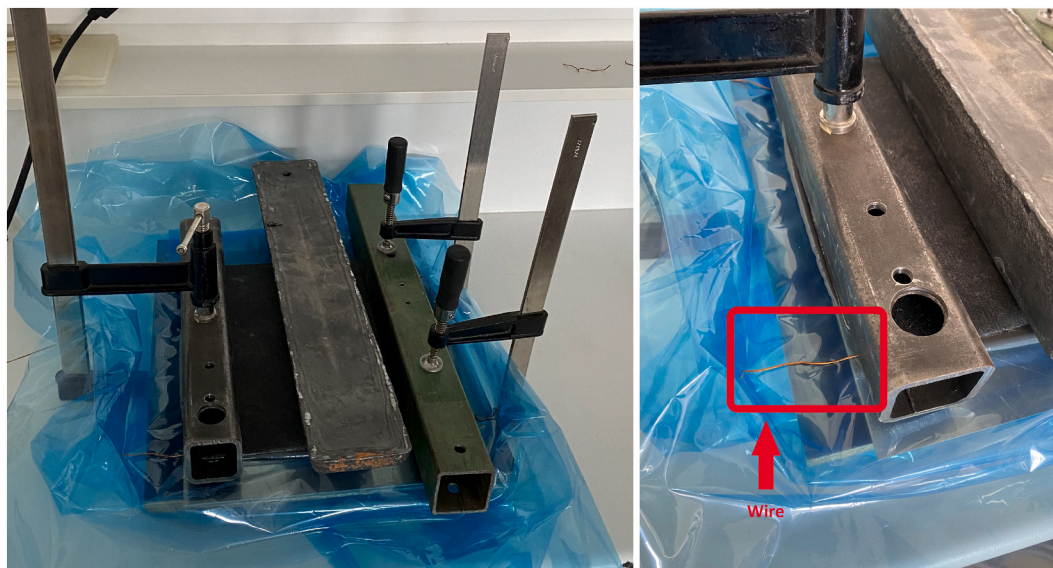
Fig. 2. Assembly set-up and adhesive thickness control.
