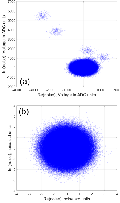
Fig. 4. Clouds of the samples from the noise range profile at the IQ plane: (a) a multimodal distribution of the measured data, (b) Gaussian distribution after application of the proposed algorithm (skewness 10^{-7} , kurtosis 3.147 for both real and imaginary parts of the signal).
