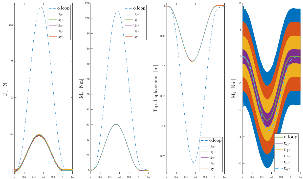
Fig. 22 Open and closed-loop response comparisons with backlash and actuator scaling parameter k = 0.5 .
