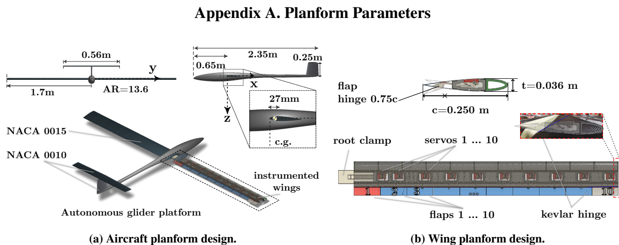
Fig. 20 Overview of the wing planform design.
