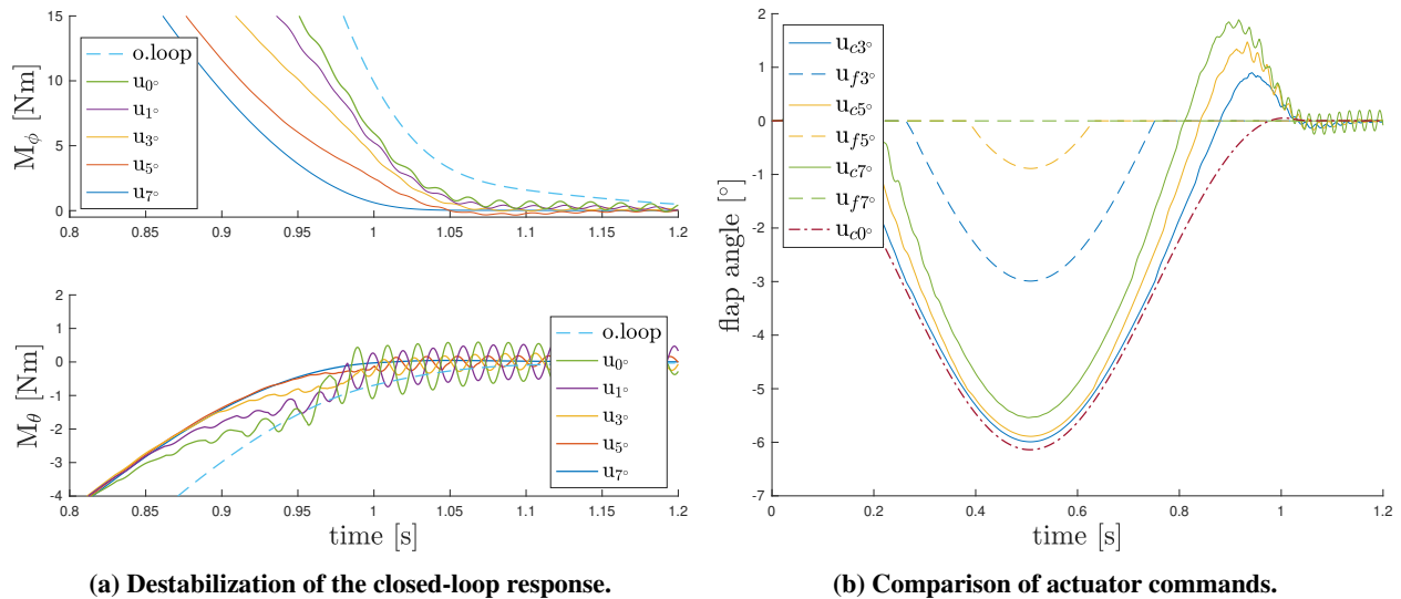
Fig. 13 Comparison responses to various degrees of free-play.
