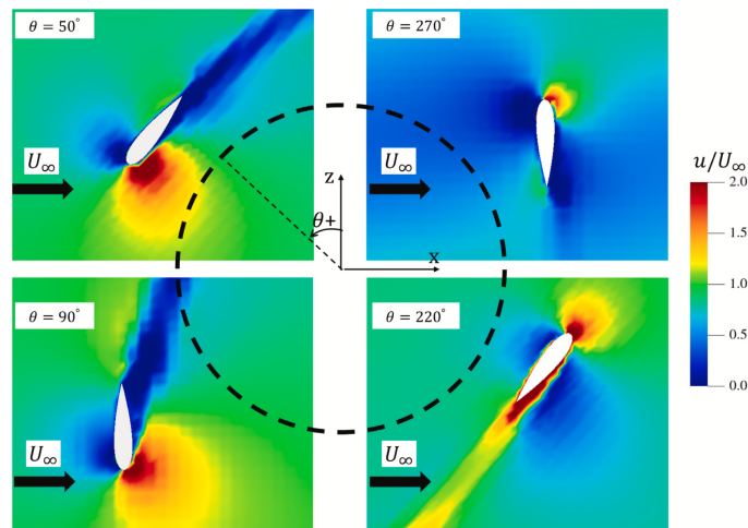
Fig. 9 Instantaneous streamwise velocities experienced by a VAWT blade at different azimuth locations as obtained by Brandtetti et al. [43]; u : streamwise velocity, U_\infty : freestream velocity (reprinted after written permission)
