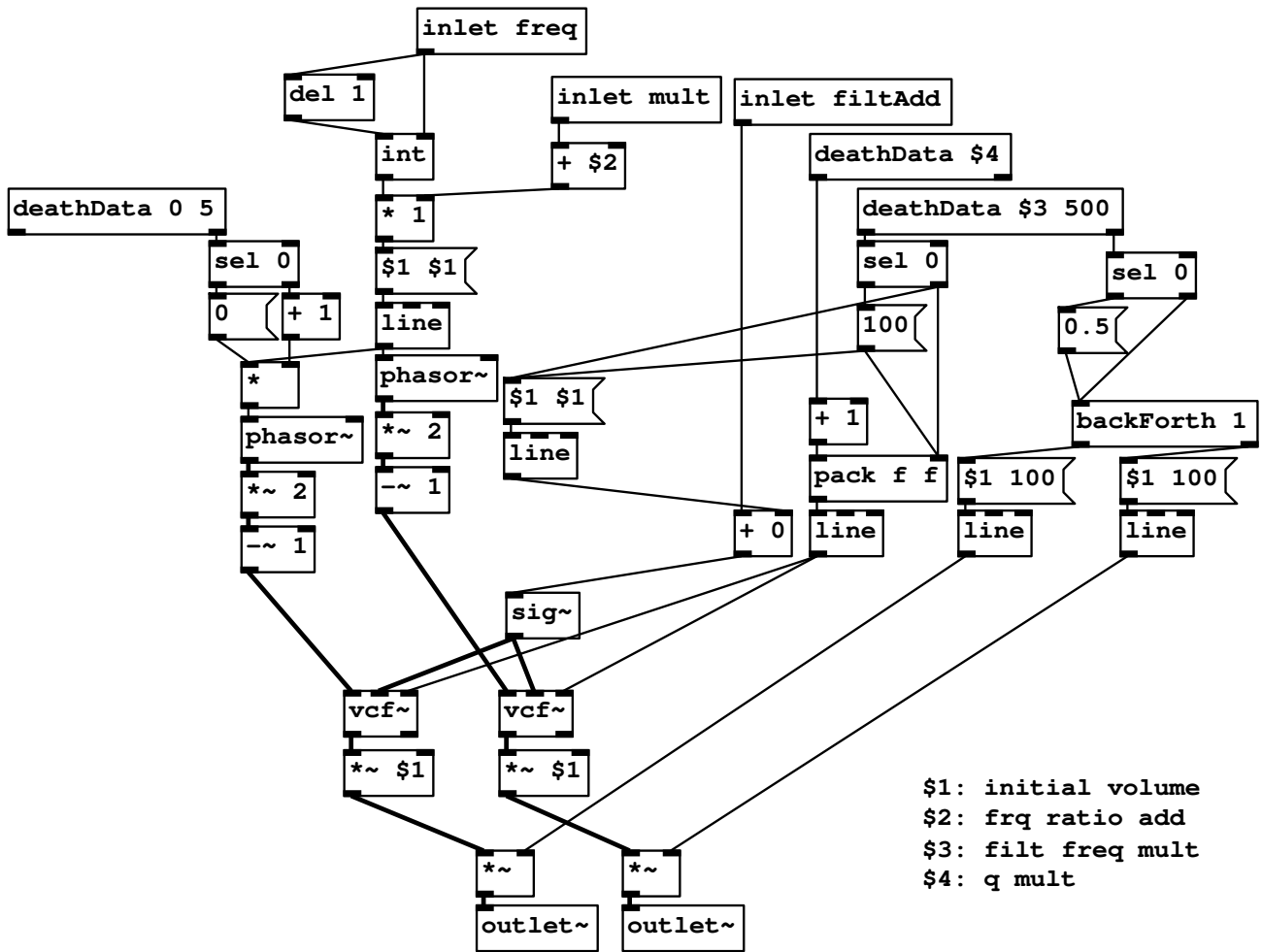
Figure 2: [subOsc~] Pd abstraction used in the Pure Covidata project
