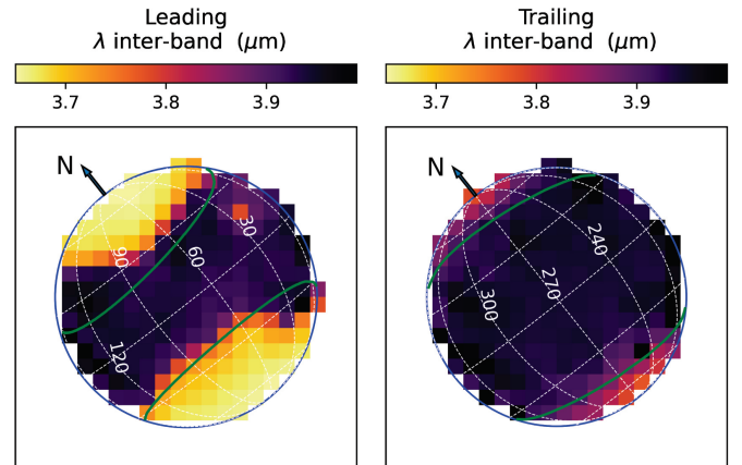
Fig. 8. Spatial variations of 3.6–3.9 \mu m inter-band properties. Inter-band amplitude A_{IB} (top) and wavelength position (bottom) for the leading (left) and trailing (right) hemispheres.
