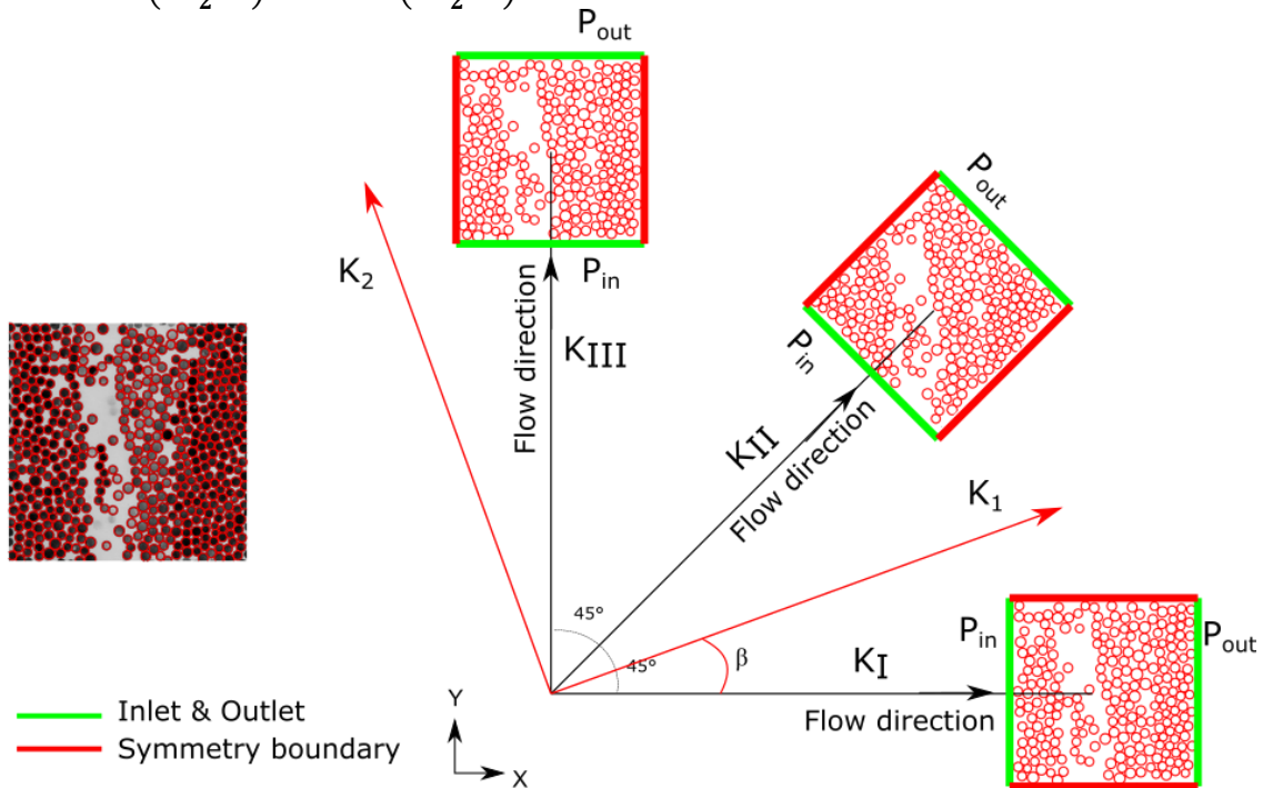
Figure 4: Schematic representation of the three directions for the 1D flow simulations to derive the principal direction and the principal permeability components.
