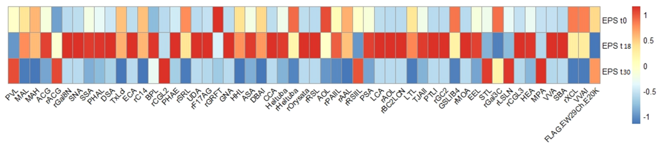
Figure 4. Lectin binding profiles of the extracellular polymeric substances extracted from aerobic granular sludge. EPS 10 : EPS extracted from inoculum; EPS t18 : EPS extracted from granules 18 days after the reactor start; EPS t30 : EPS extracted from granules 30 days after the reactor start. The scale ranges from 1 to –1. Red: high intensity; blue: low intensity.
