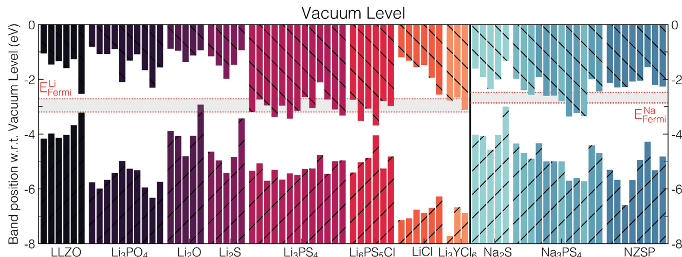
Figure 4. Alignment of SE surfaces versus Li and Na metal references indicated by the gray areas enclosed in red dotted borders. The y -axis is the energy level relative to the vacuum level of each SE, with y = 0 indicating the vacuum level. The upper bars are the conduction band minima, and the bottom bars are the valence band maxima of each SE. NZSP refers to NaSICON \text{Na}_3\text{Zr}_2\text{Si}_2\text{PO}_{12} .
