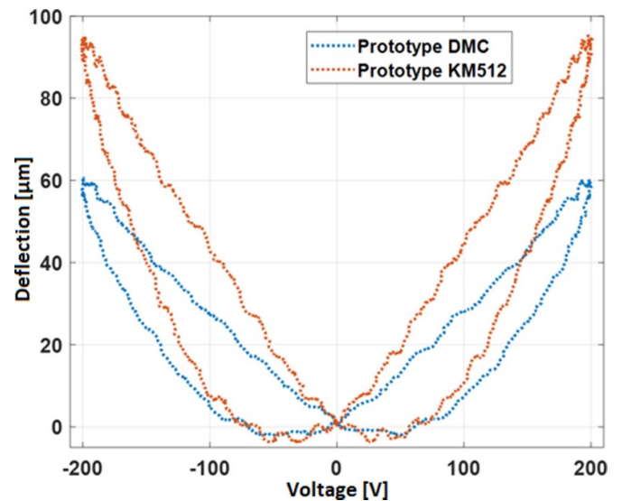
Figure 18. Actuation hysteresis under a 1 Hz 200 V bipolar sinusoidal excitation.
