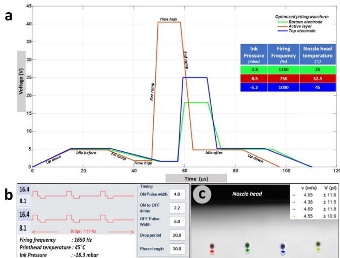
Figure 3. Jetting the ink droplets: (a) waveforms for jetting the conductive and EAP inks on the Dimatix DMC-11610 printhead; (b) waveform for jetting the EAP ink on the Konica Minolta KM512 printhead; and (c) analysing the EAP ink jetting in the DropView software module (Pixdro LP50).
