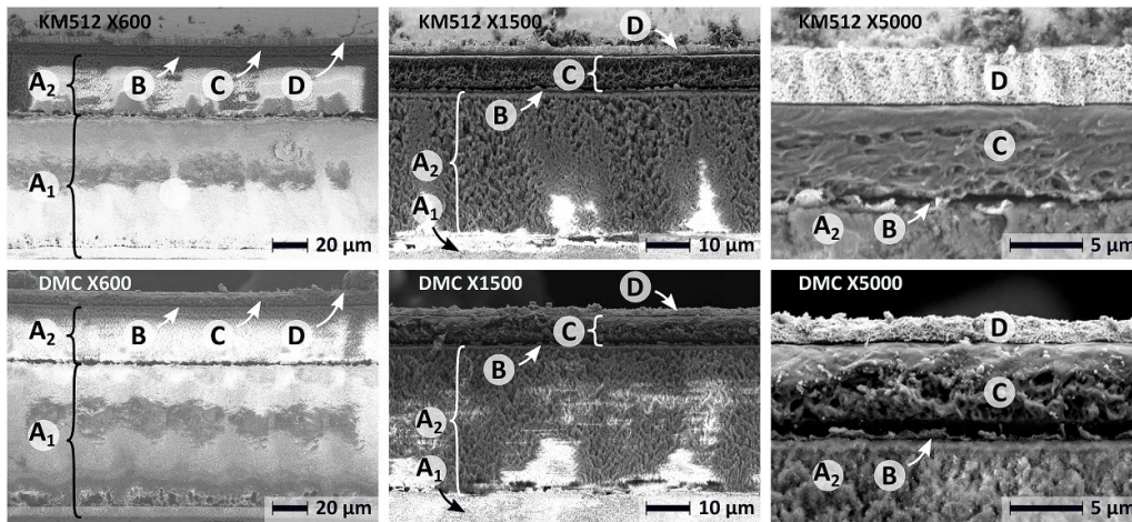
Figure 14. SEM images of the actuator cross-sections (JEOL JSM 6010LA): a KM512 sample in the top row, and a DMC sample in the bottom row. A —Novole IJ-220 PEN substrate ( A 1 ) with the microporous resin coating ( A 2 ); B —bottom electrode; C —P(VDF-TrFE-CTFE) layer; and D —top electrode.
