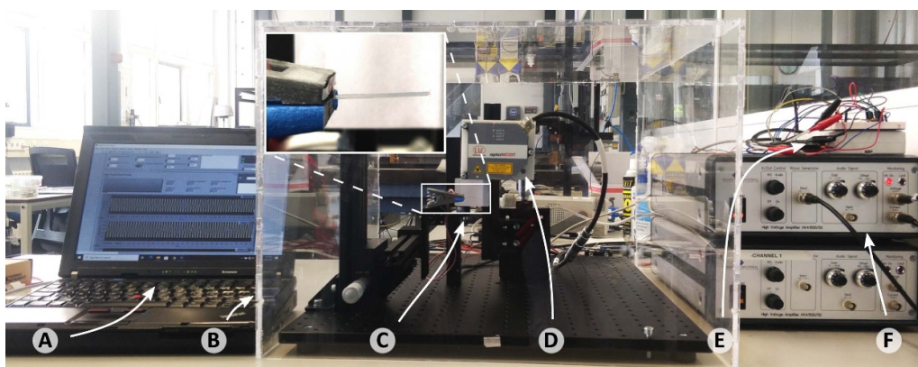
Figure 12. The experimental set-up for actuation performance characterisation: A —PC with the NI LabView environment; B —transparent acrylic box; C —clamped actuator; D —laser displacement sensor; E —data acquisition system; and F —high-voltage power amplifier.
