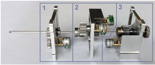
Fig. 5. The drive separated in its three modules.
