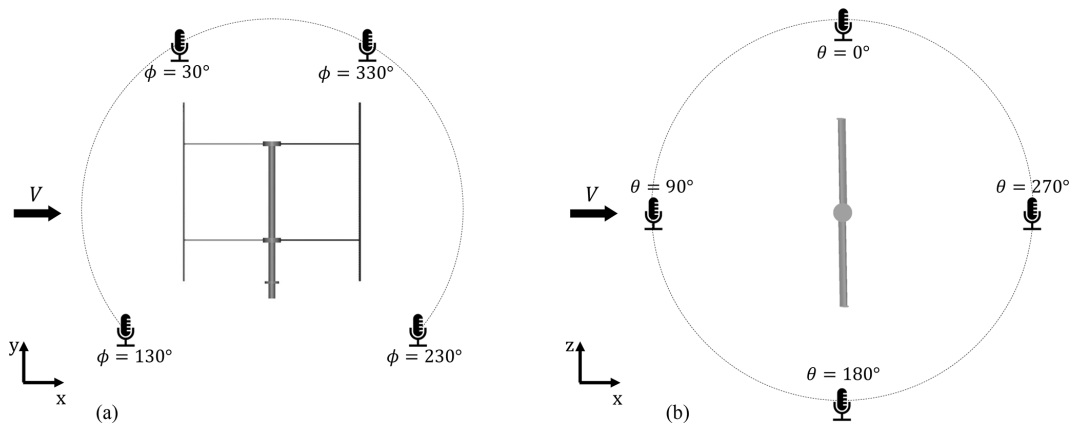
Figure 7. Two circular arrays of virtual microphones are positioned at a distance of 2.6D from the centre of the VAWT. Array (a) comprises four microphones located in the x – y plane, while array (b) consists of four microphones positioned in the x – z plane. These locations are considered relevant for characterising the psychoacoustic annoyance of the sound source.
