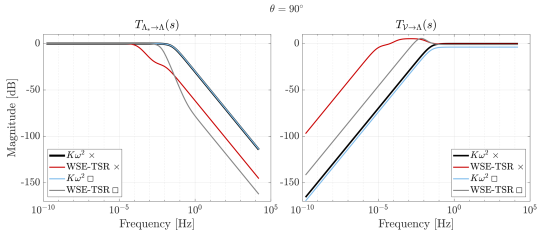
Figure 13. Bode plots of the closed-loop transfer functions T_{\Lambda_* \rightarrow \Lambda}(s) and T_{V \rightarrow \Lambda}(s) for the baseline K\omega^2 and the WSE-TSR tracking controllers. The MCDM solutions for the WSE-TSR tracking controller reveal that the reference tip-speed ratio tracking and disturbance rejection capabilities have to be offset to achieve a 39 % increase in power production, for the \times case, and a 25 % reduction in actuation effort, at the cost of 2 % power decrease and 6 % increase in psychoacoustic annoyance, for the \square case, compared to the K\omega^2 controller.
