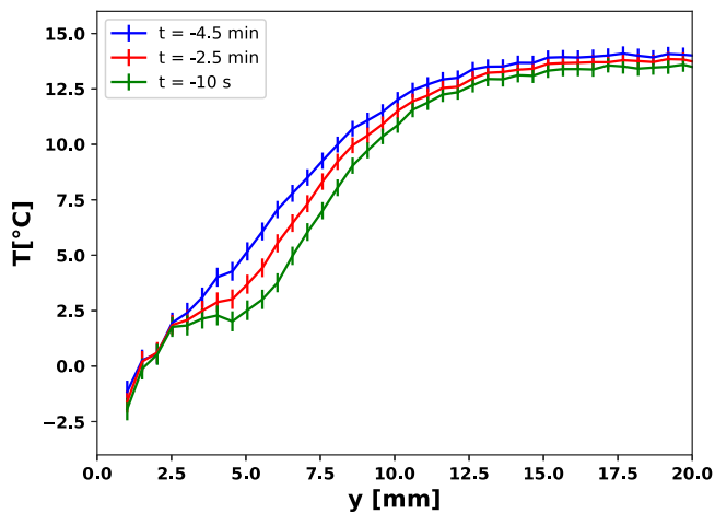
Fig. 11. LIF temperature profiles for T_{in,set} = 15^\circ\text{C} at the center of the channel ( x = 75\text{ cm} ), taken for various times prior to the onset of ice formation.
